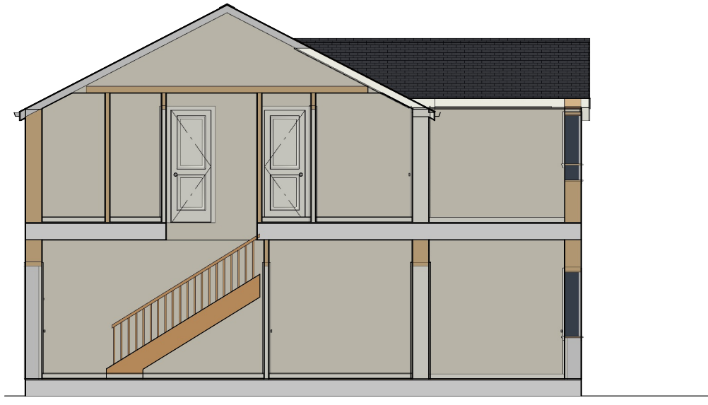
Proposed second side elevation
