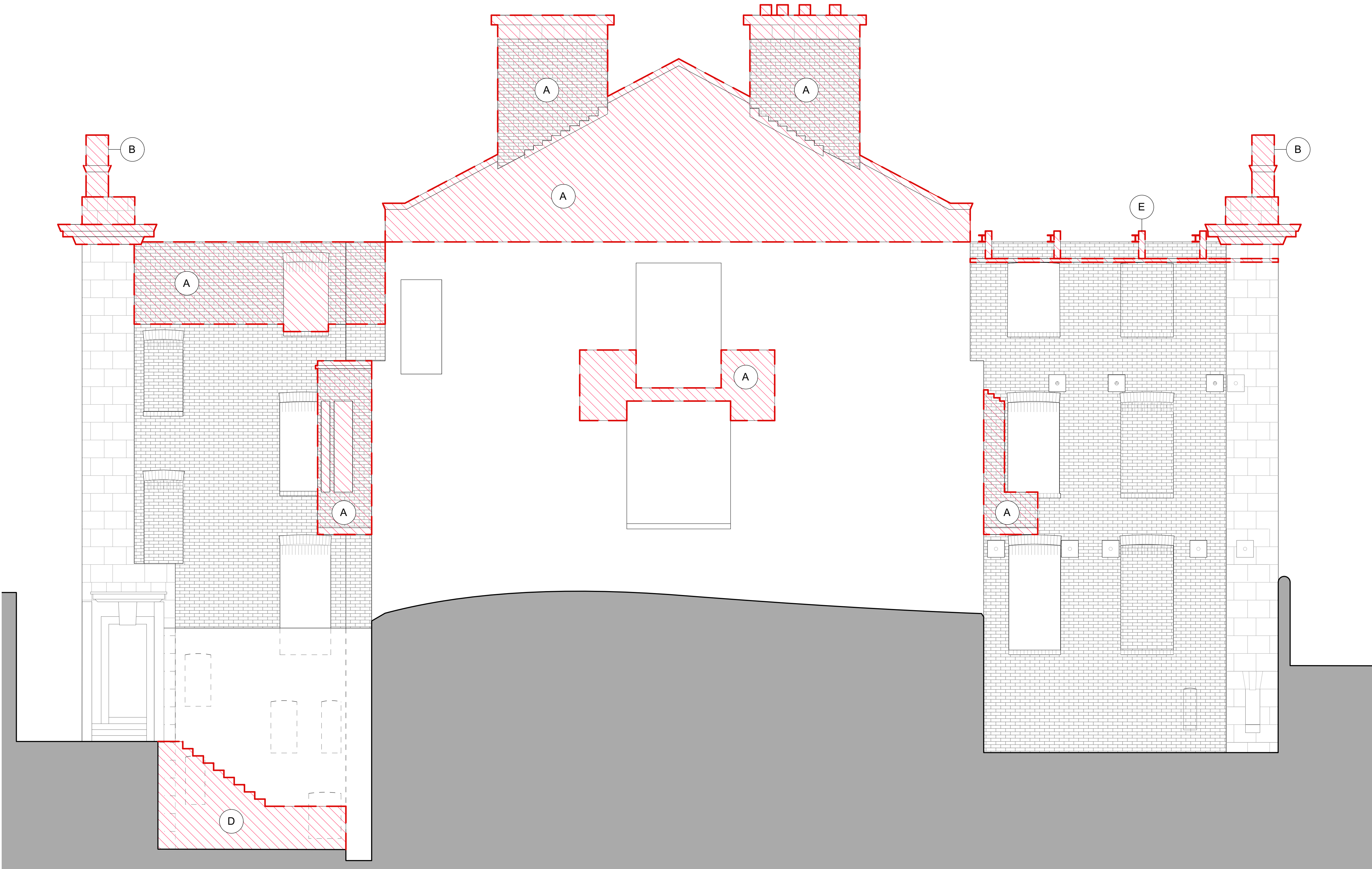
1 North Demolition Elevation Scale: 1:50
