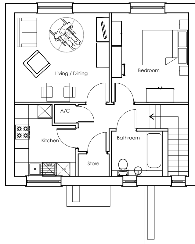
FIRST FLOOR PLAN (53m2 / 570sq.ft.)
