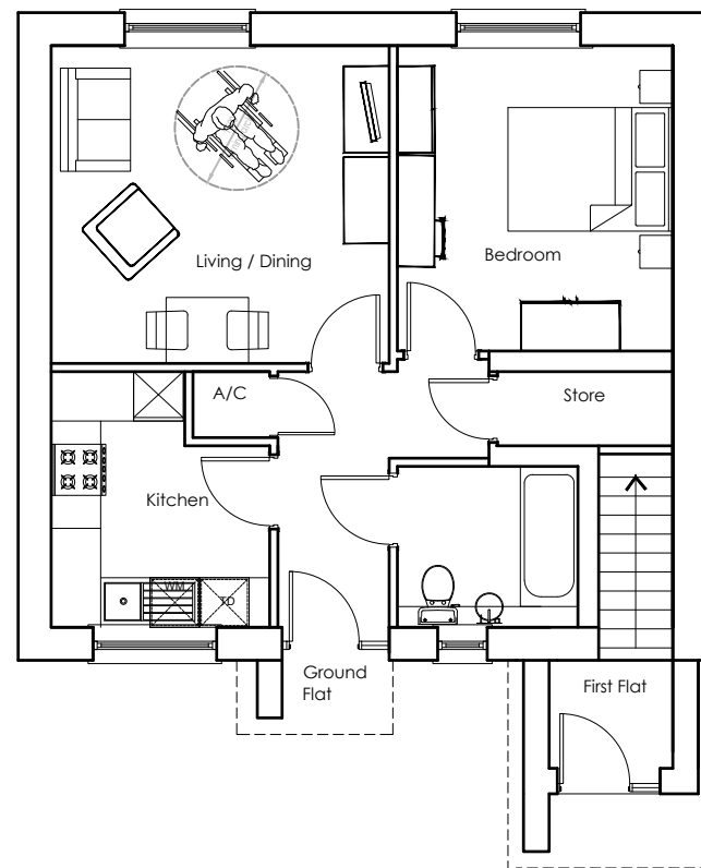
GROUND FLOOR PLAN (50m2 / 538sq.ft.)
