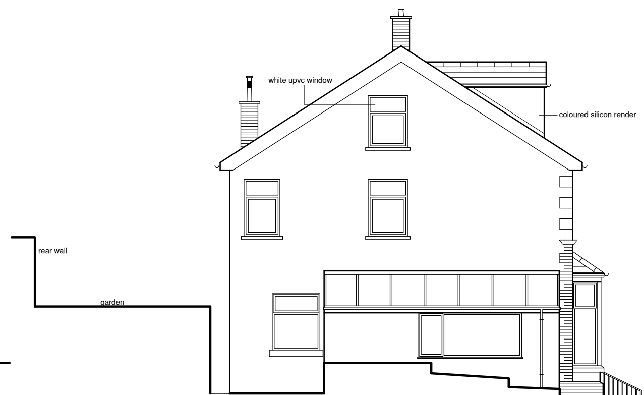
SIDE ELEVATION
