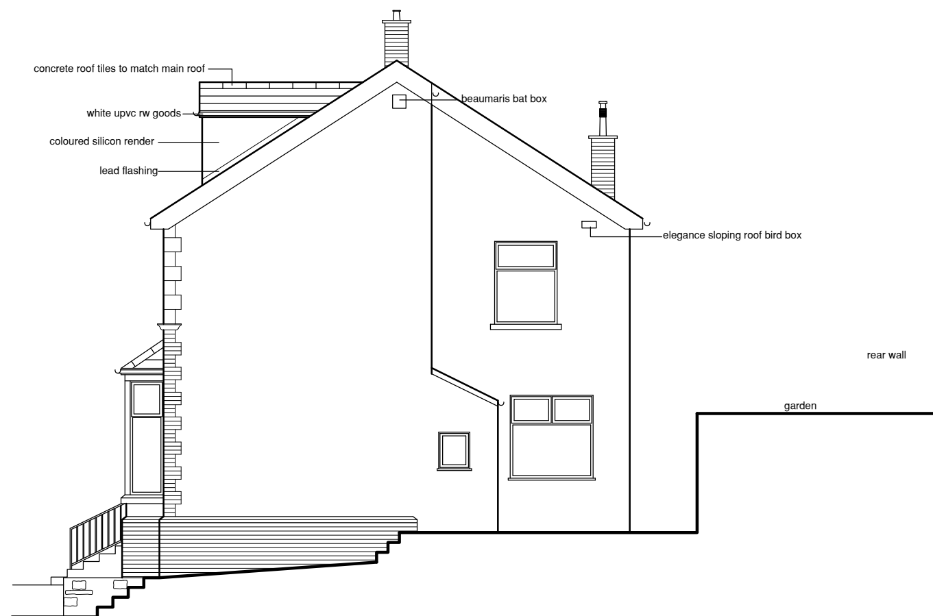
SIDE ELEVATION
