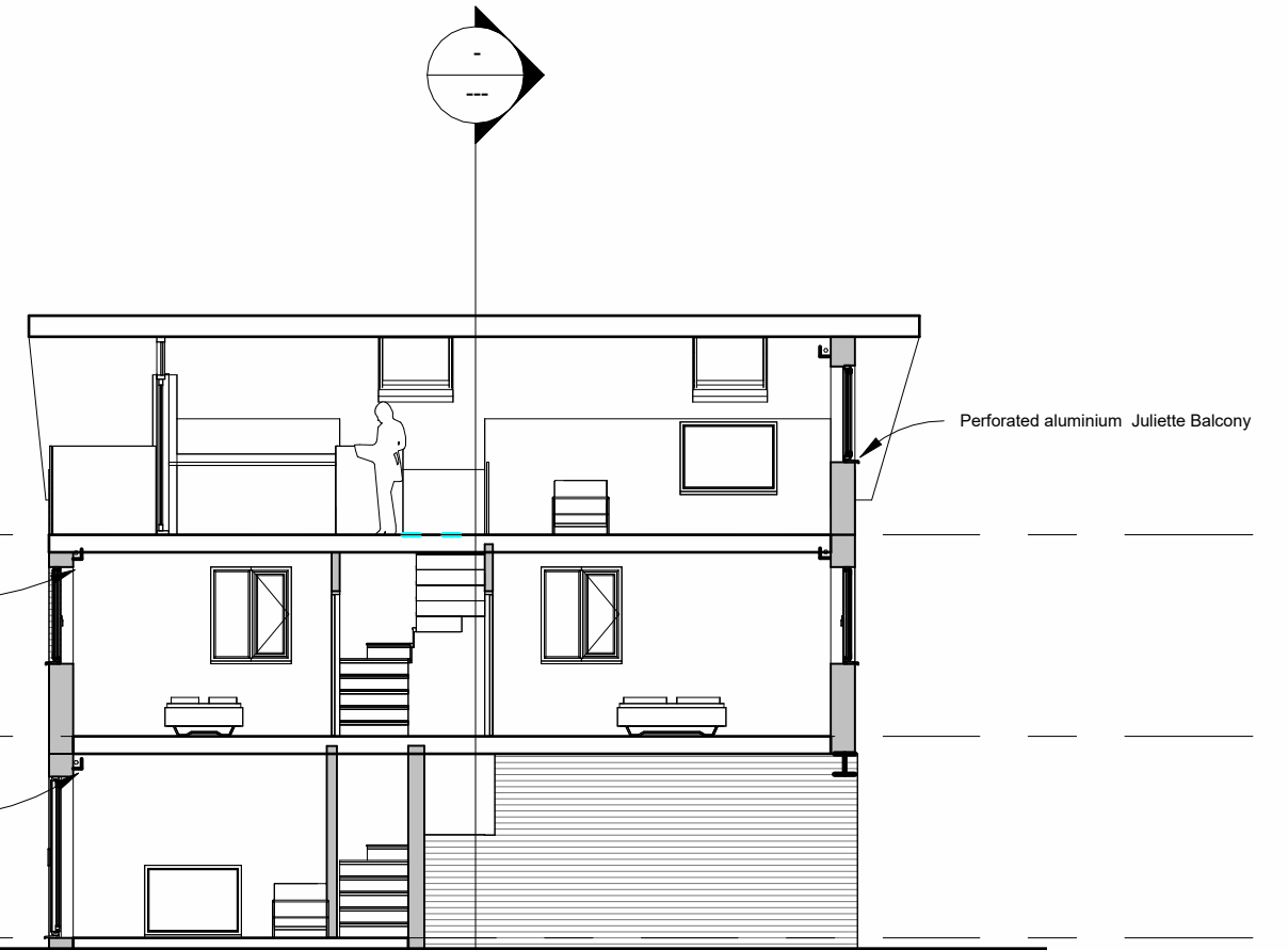
Section 1
