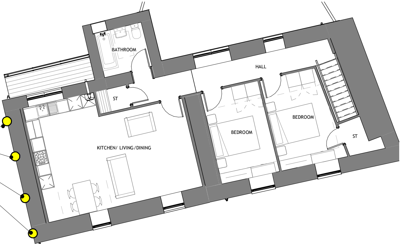
03 PROPOSED LOWER GROUND TO NO.25 (BIN STORE) 1 : 100
