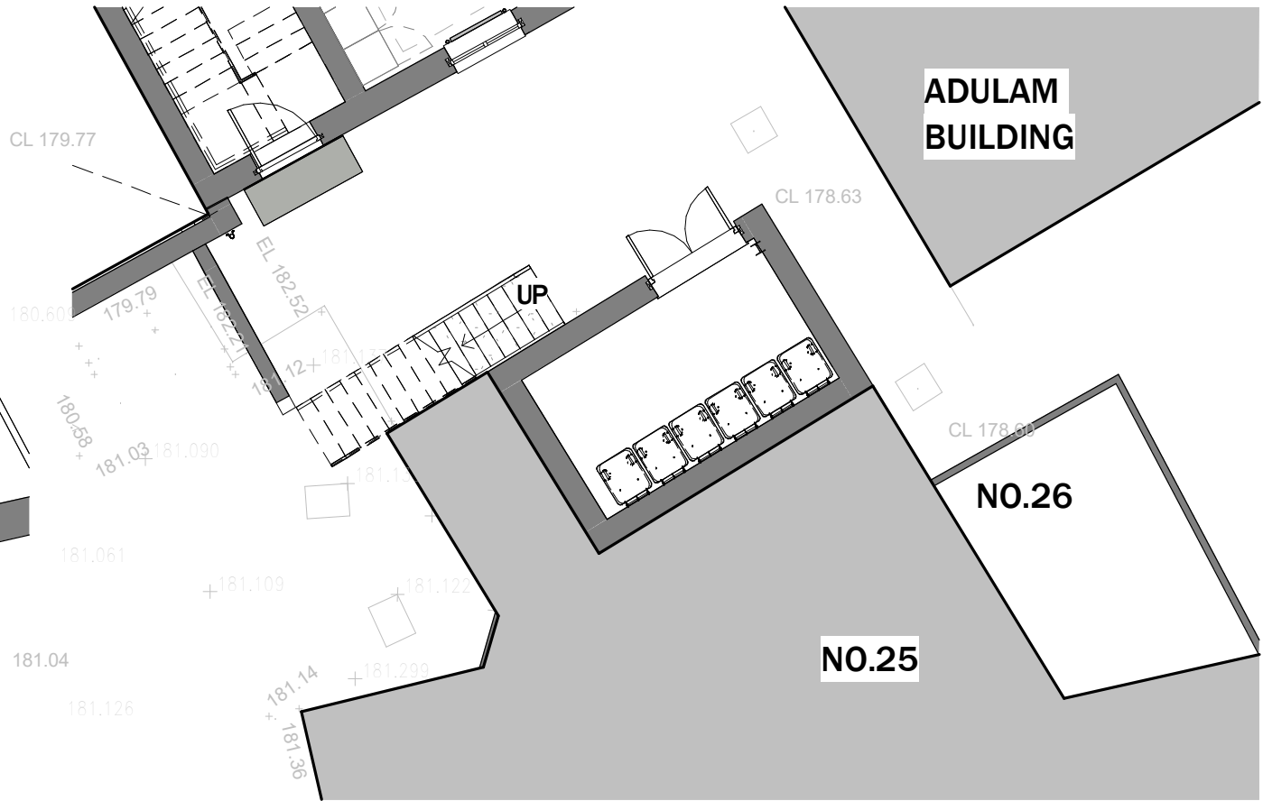
03 PROPOSED LOWER GROUND TO NO.25 (BIN STORE) 1 : 100
