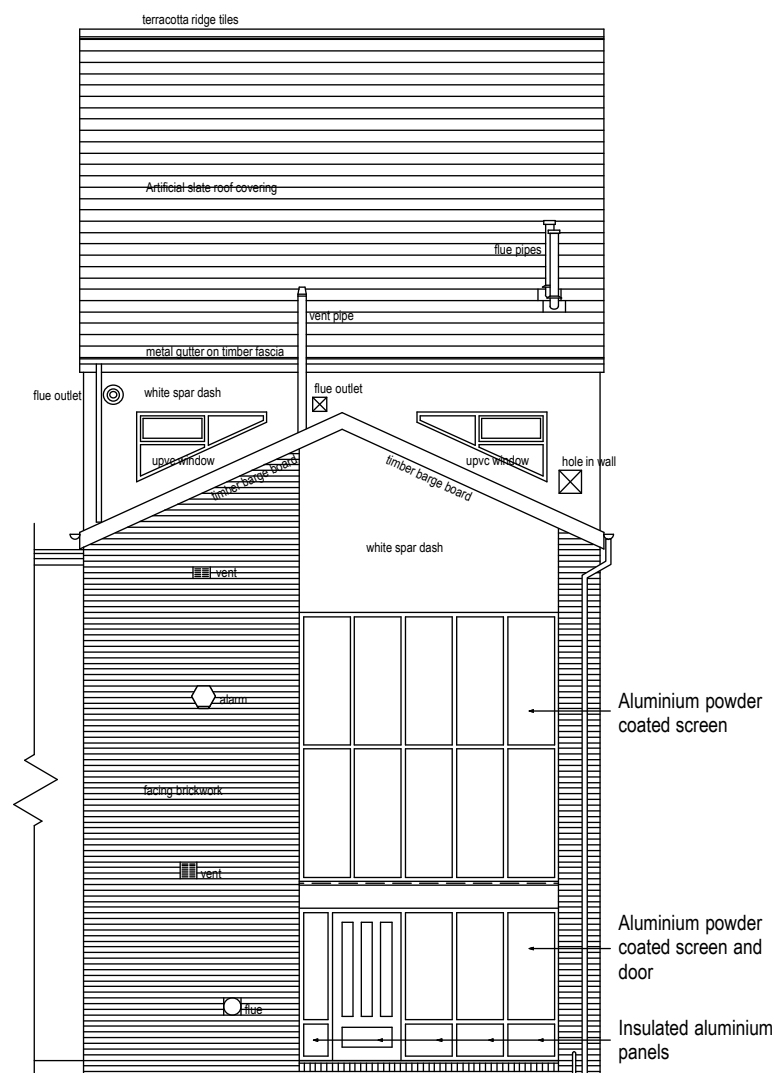
PROPOSED REAR ELEVATION 1:100
