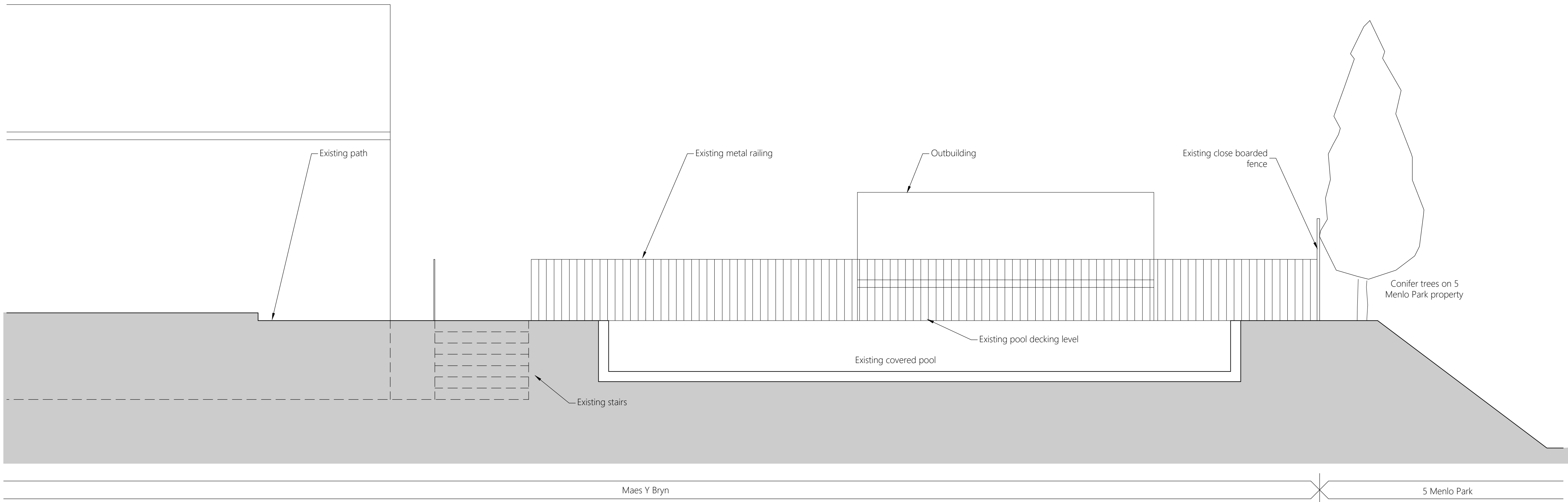
1 Existing Site Section 3 1:50 @ A1
