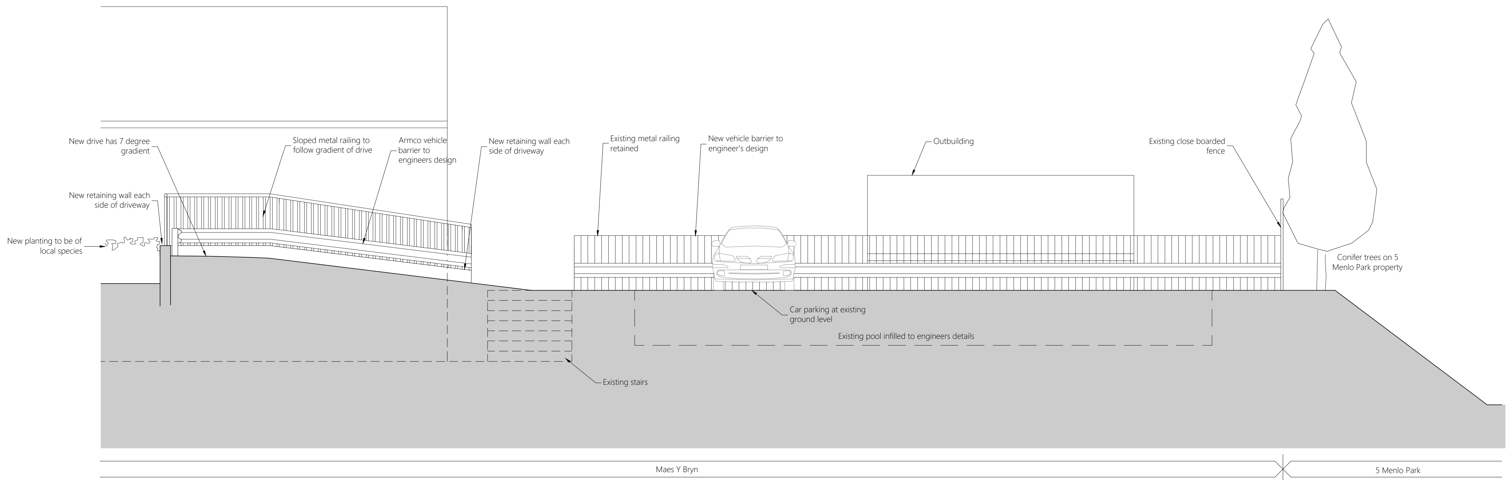
2 Proposed Site Section 3 1:50 @ A1
