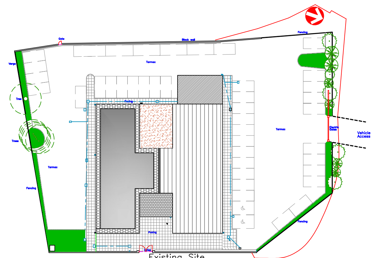
Existing Site Plan 1:500
