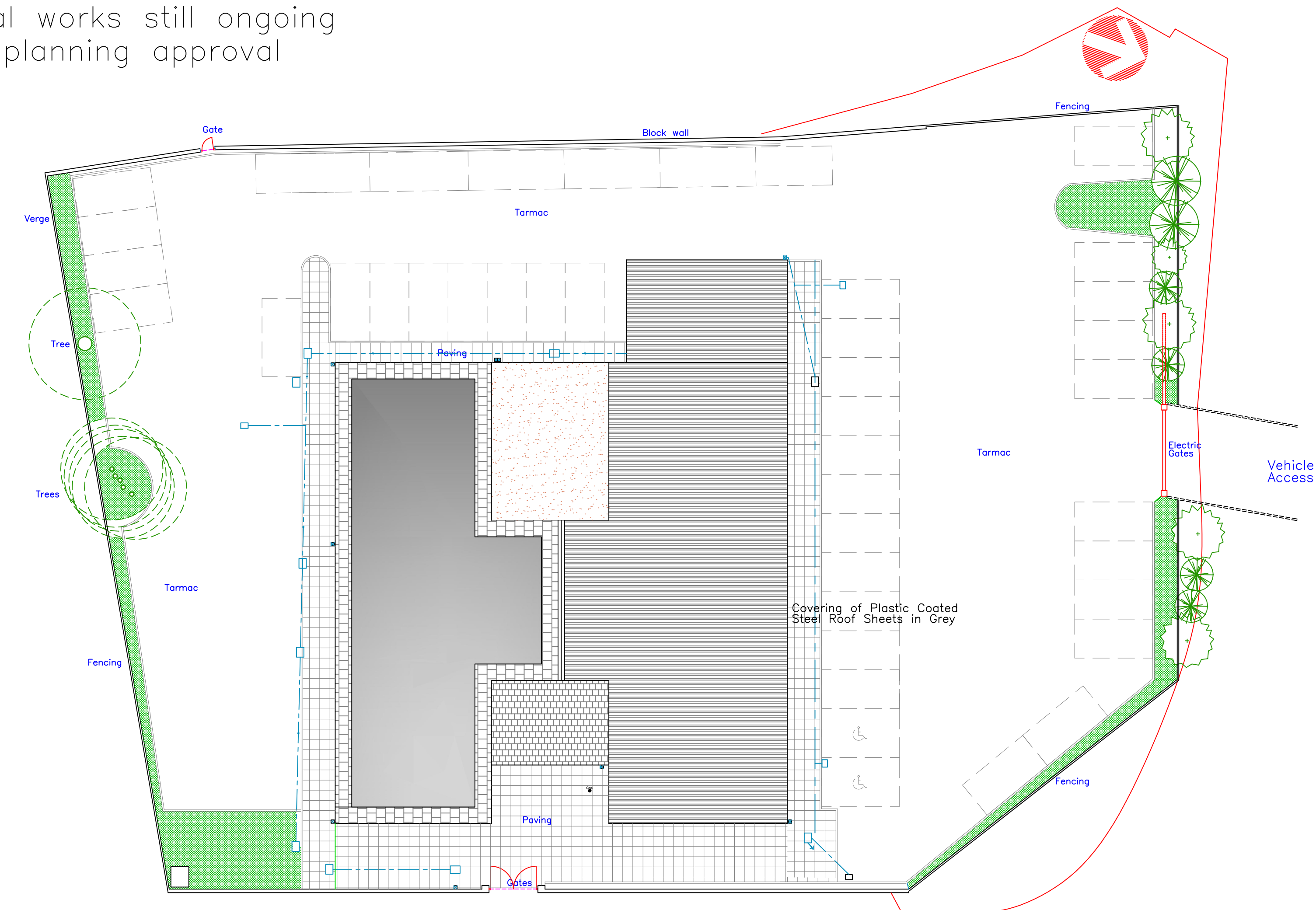
Proposed Site Plan 1:200
