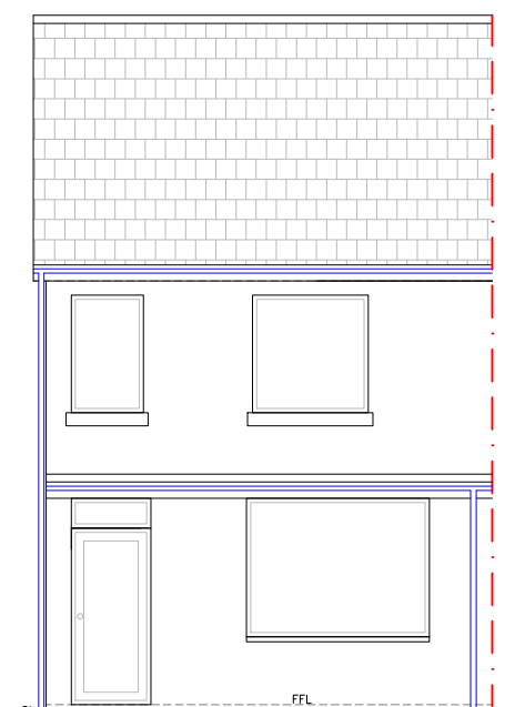
Existing Front Elev 1:100
