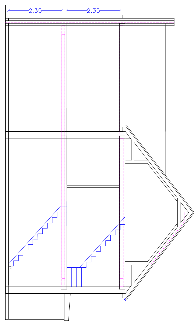
Proposed Section 1:100
