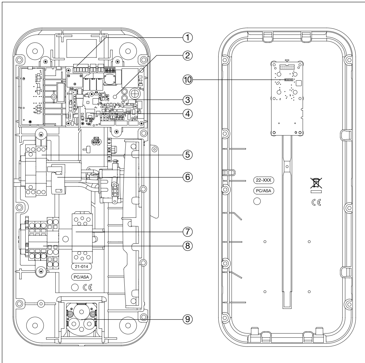
Fig. 3: Interior view of the witty charging station
