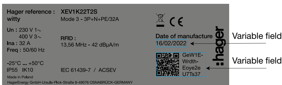
Fig. 1: Type label of the witty charging station
