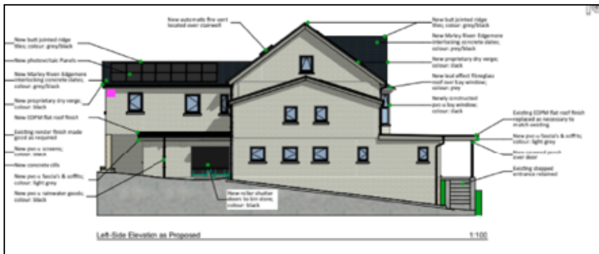
South Western Elevation
