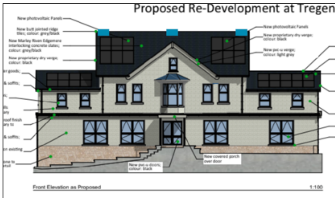
South Eastern Elevation
