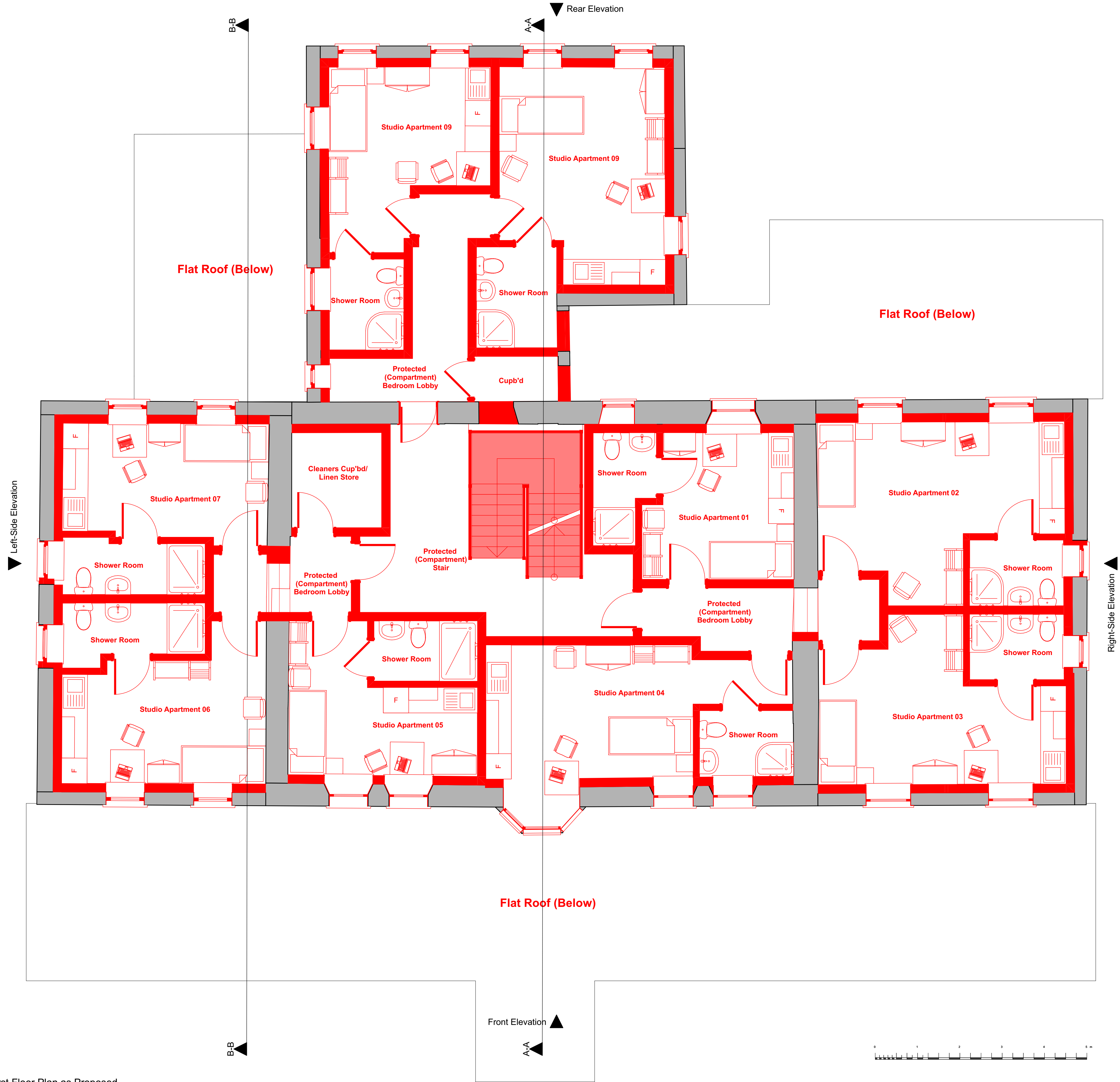
First Floor Plan as Proposed
