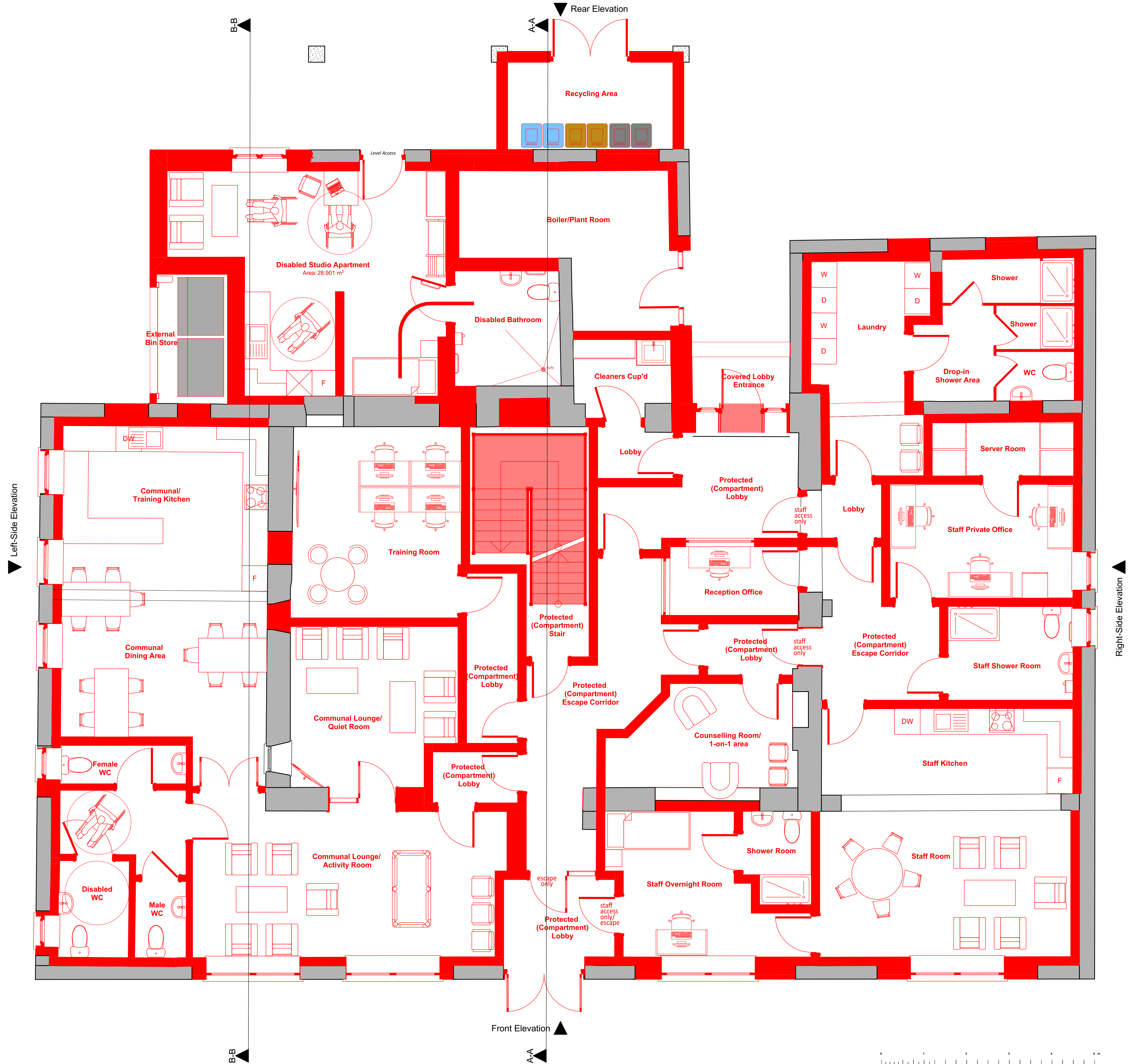
Ground Floor Plan as Proposed
