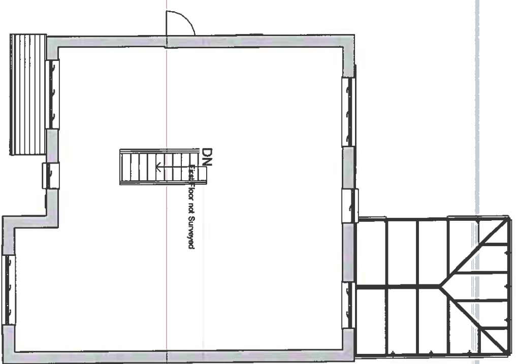
2 Existing First Floor 1 : 100
