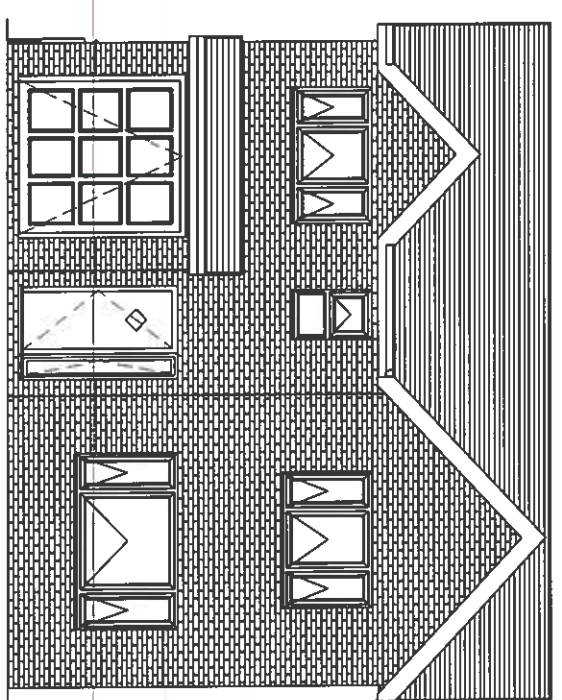
3 Existing Front Elevation 1 : 100
