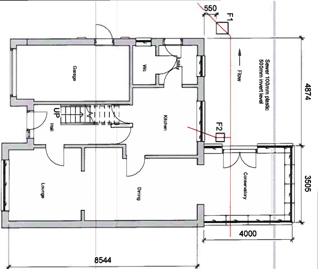
1 Existing Ground Floor 1 : 100
