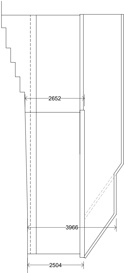
SIDE ELEVATION
