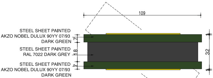
PLAN VIEW 1/20
