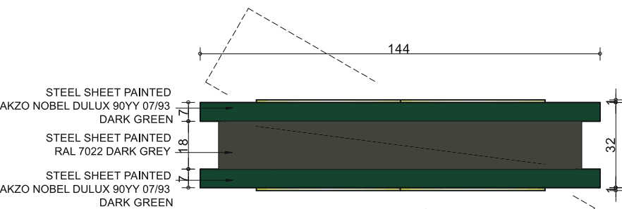
PLAN VIEW 1/20
