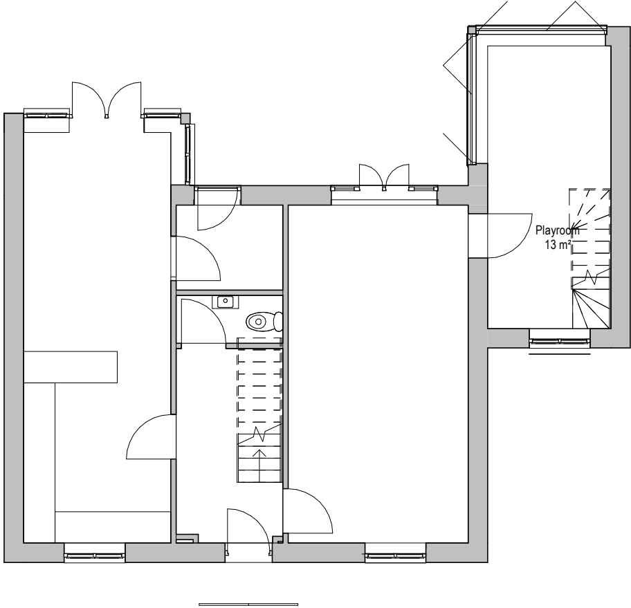
Ground Floor Proposed ( 1 : 100)
