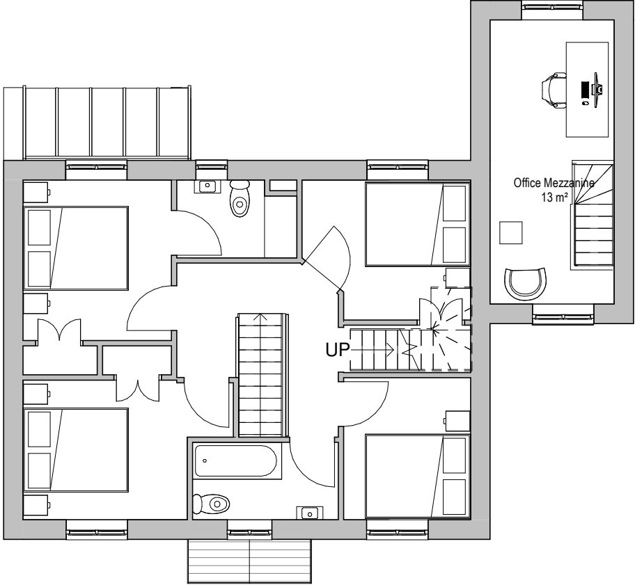
First Floor Proposed ( 1 : 100)
