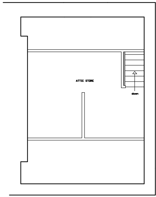
PROPOSED ATTIC FLOOR PLAN
