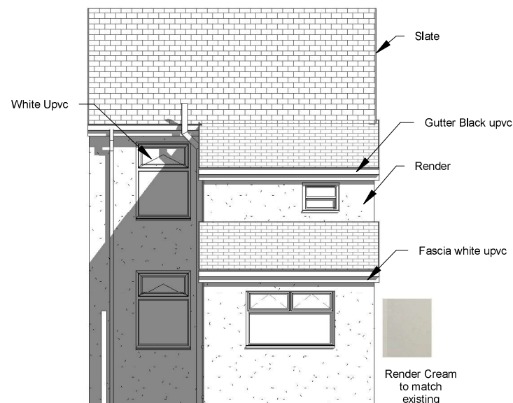
3 Existing Rear Elevation 1 : 100
