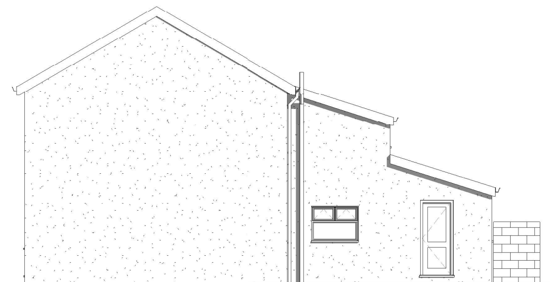
5 Existing Side 2 Elevation 1 : 100
