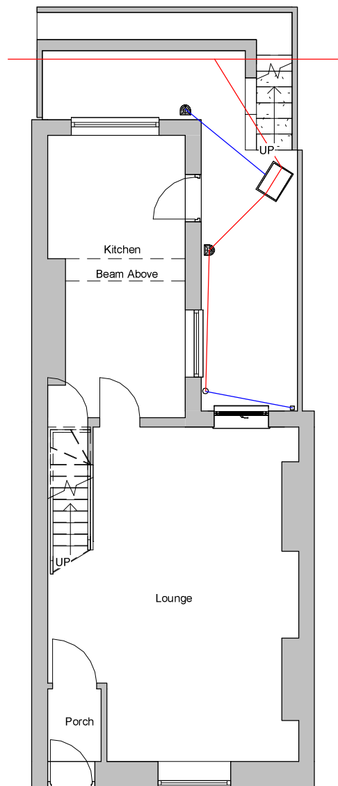
1 Existing Ground Floor 1 : 100
