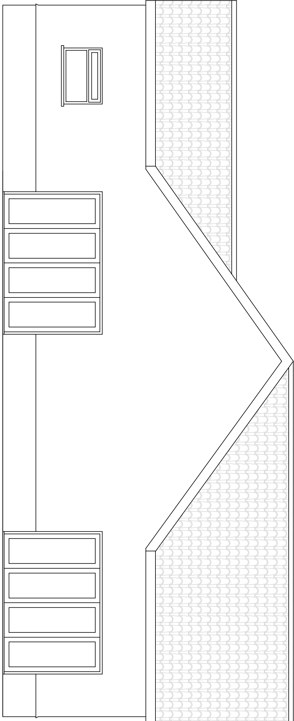
PROPOSED SIDE ELEVATION SCALE 1:50
