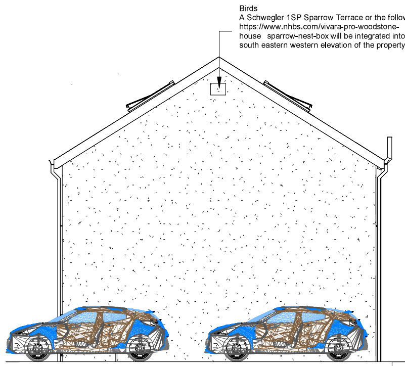
3 Side 1 Elevation 1 : 100
