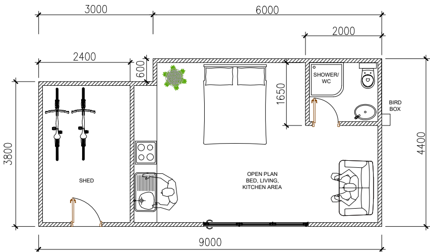
PROPOSED FLOOR PLAN
