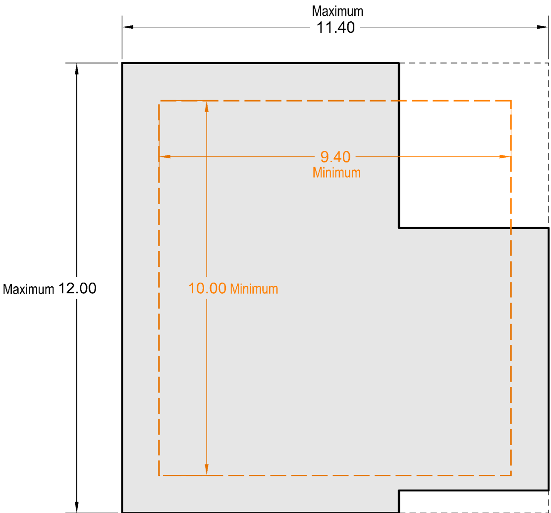
HOUSE 1 PLAN
