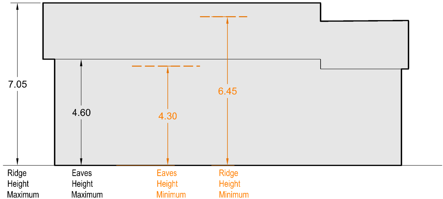
HOUSE 2 ELEVATION
