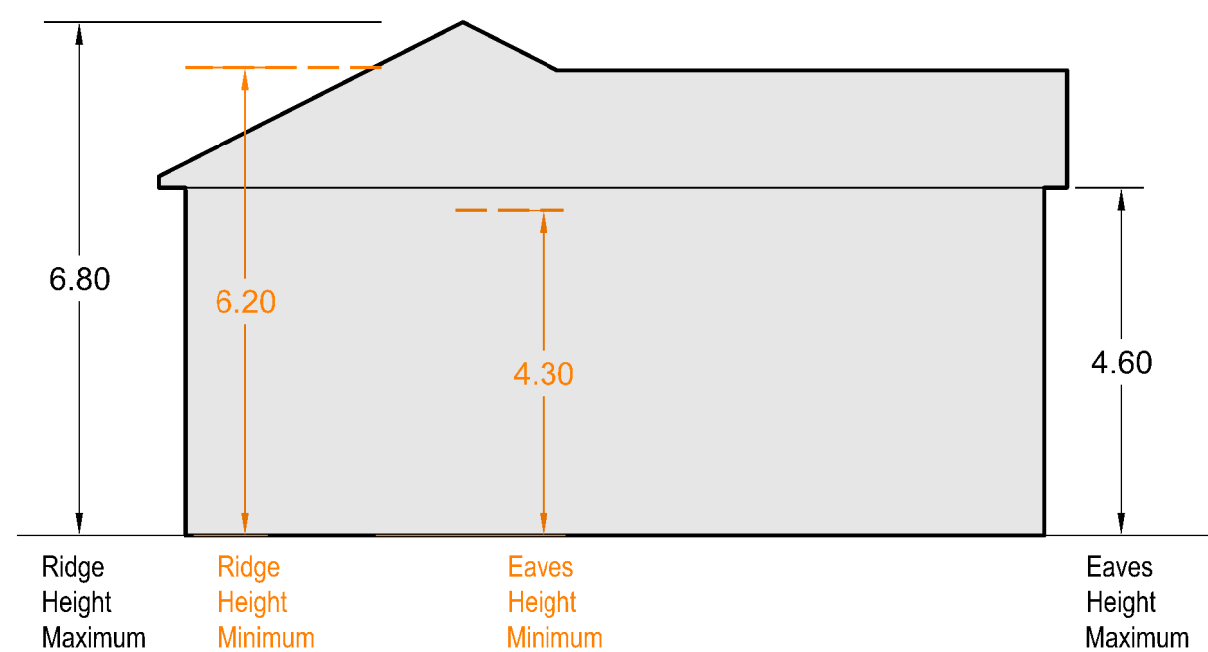
HOUSE 1 ELEVATION
