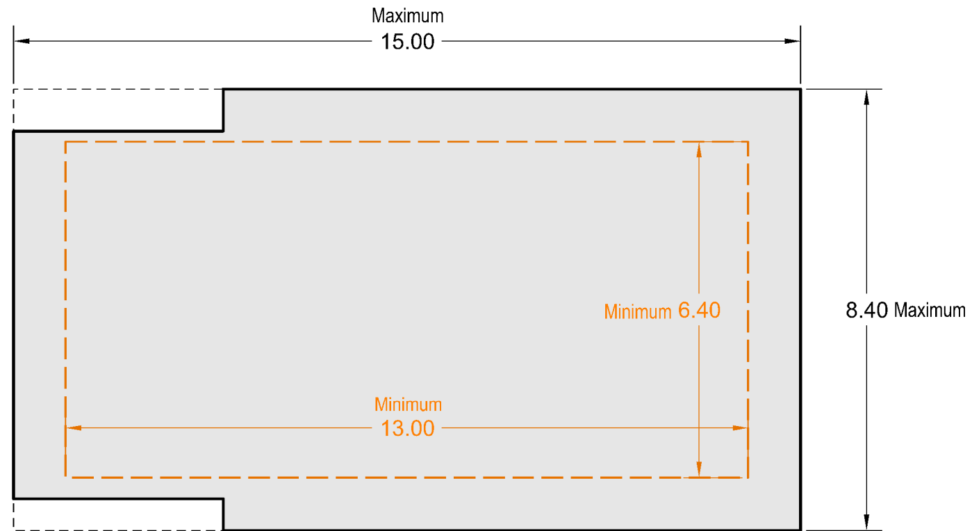
HOUSE 2 PLAN
