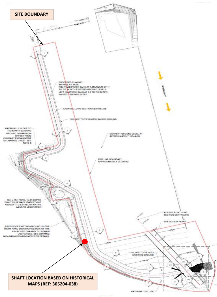
FIGURE 2: SITE PLAN
