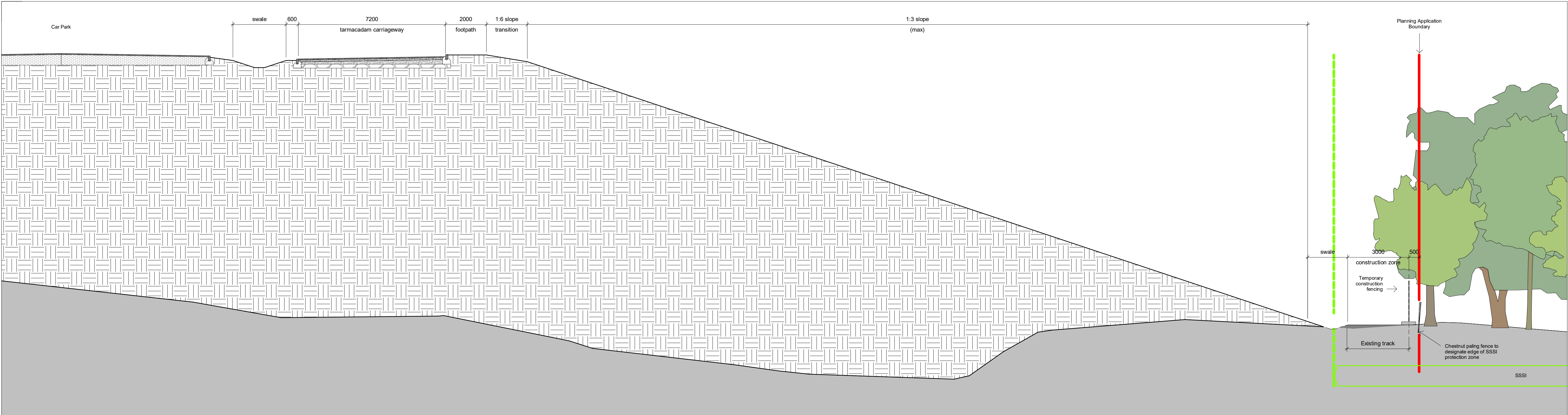
Section 10 - Resort Access Road 3 1 : 100
