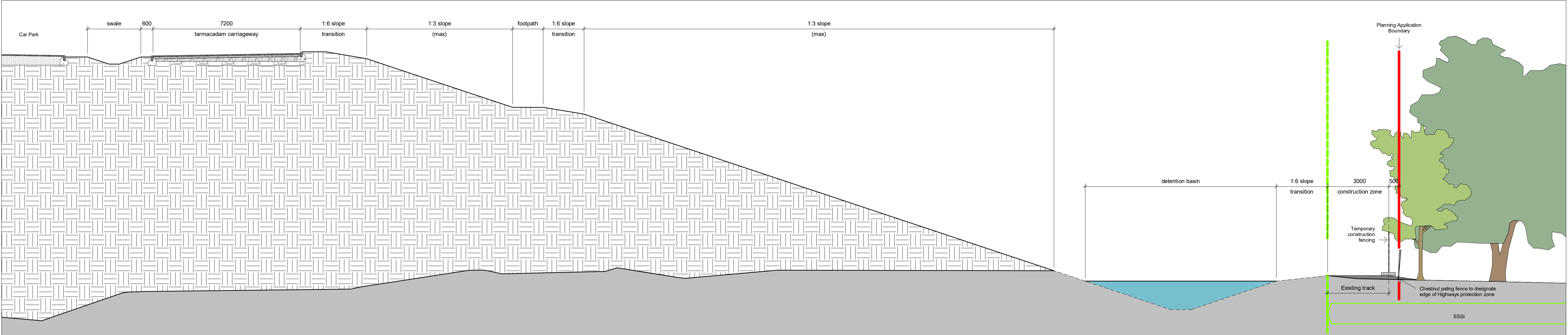
Section 9 - Resort Access Road 2 1 : 100
