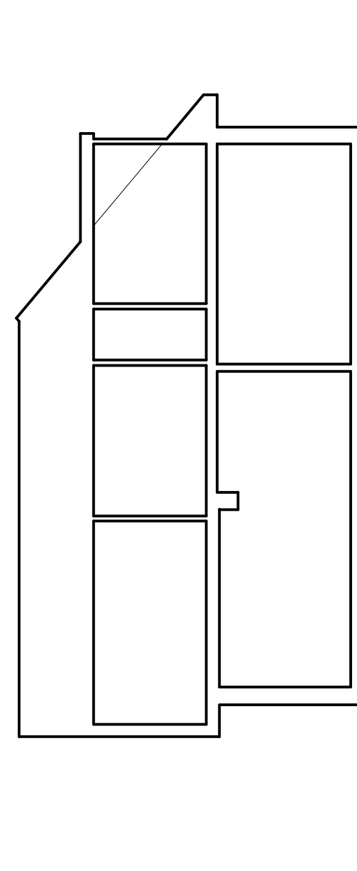
PROPOSED SECTION
