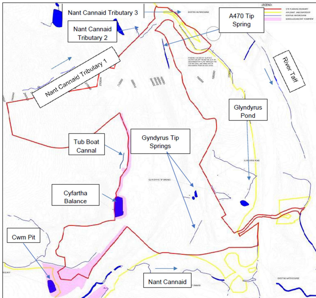
Figure 13.3.1a – Watercourse Features Watercourses Summary
