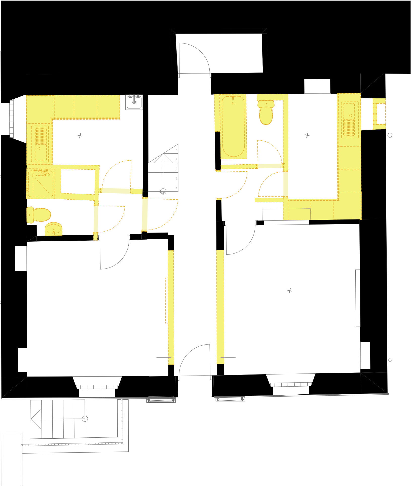
Demolition Ground Floor Plan
