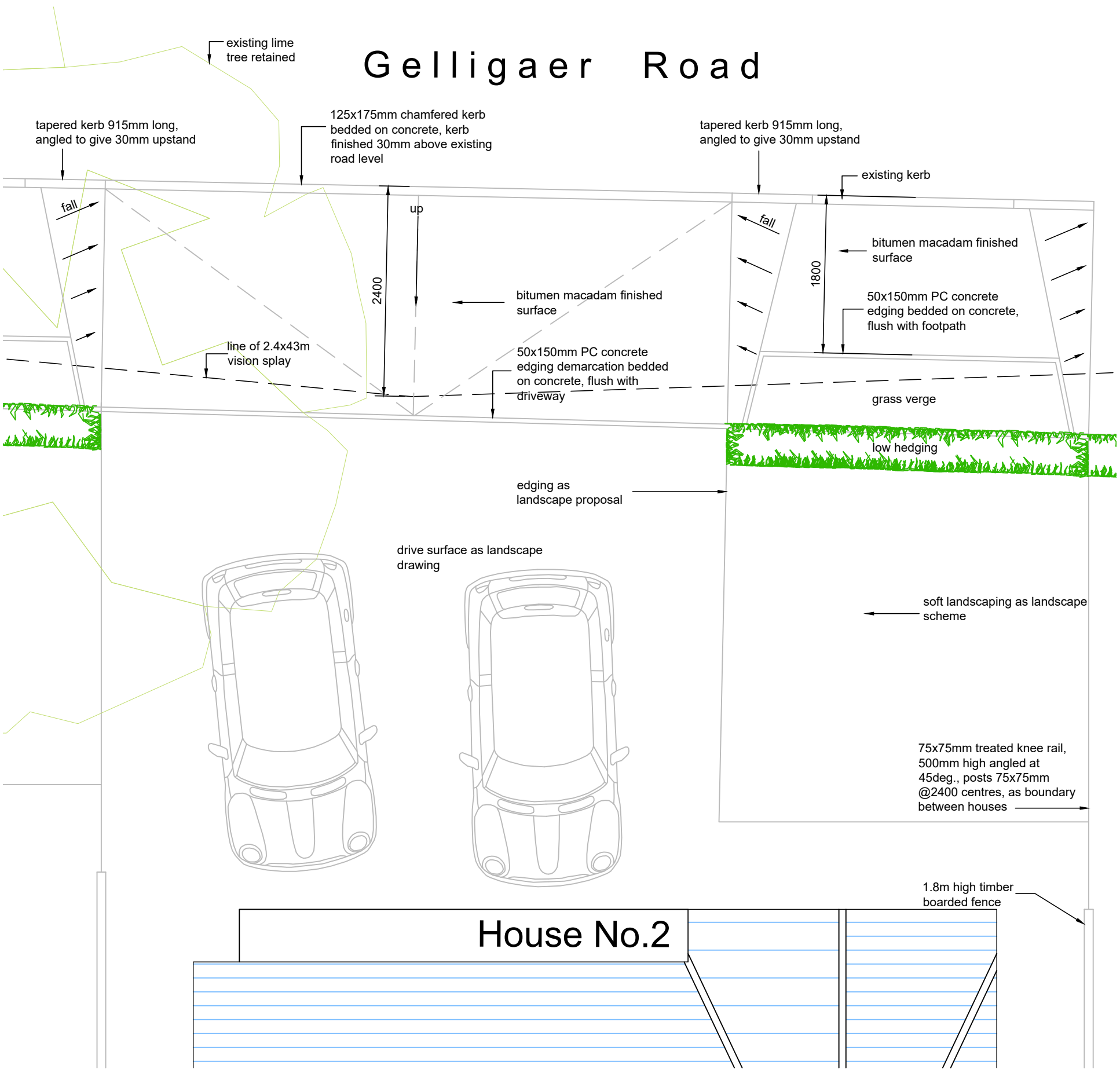
Typical Crossover/ Plan Scale 1:50
