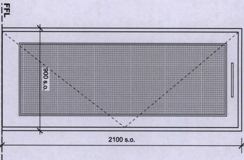
01: New external door to courtyard Elevation -ED05, outward opening, single leaf swing. -PPC finish to frame (colour TBC). L20/485
