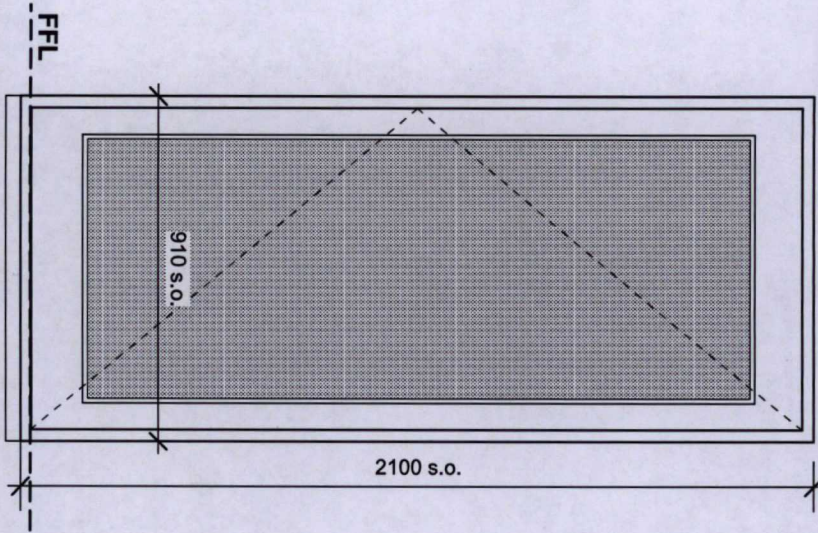
01: New external door to courtyard Elevation -ED05, outward opening, single leaf swing. -PPC finish to frame (colour TBC). L20/485
