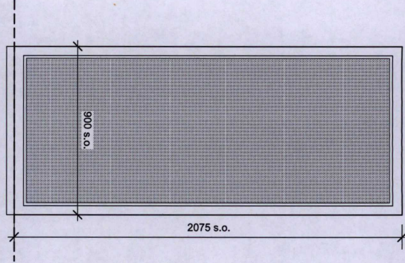
03: New external glazed screen to escape stair Elevation -WG04, fixed glazed screen -PPC finish to frame (colour TBC) -30mins fire rating (insulation and integrity). L10/330
