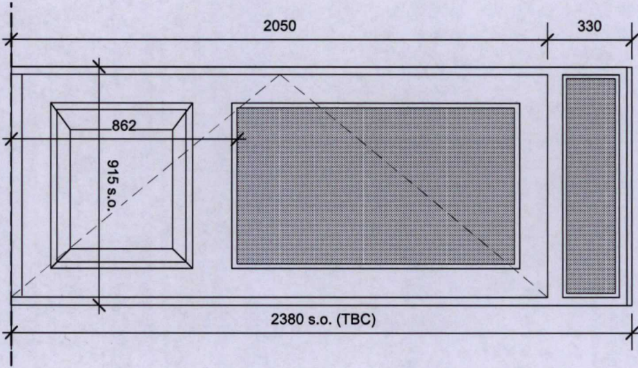
06: New external glazed door to shopfront Elevation -ED01, inward opening, single leaf swing -Timber panel to lower section, fixed glazed fanlight screen above. -Flush threshold for DDA access compliance -To achieve minimum 775mm clear width -Painted finish to door and frame (colour TBC). L20/270
