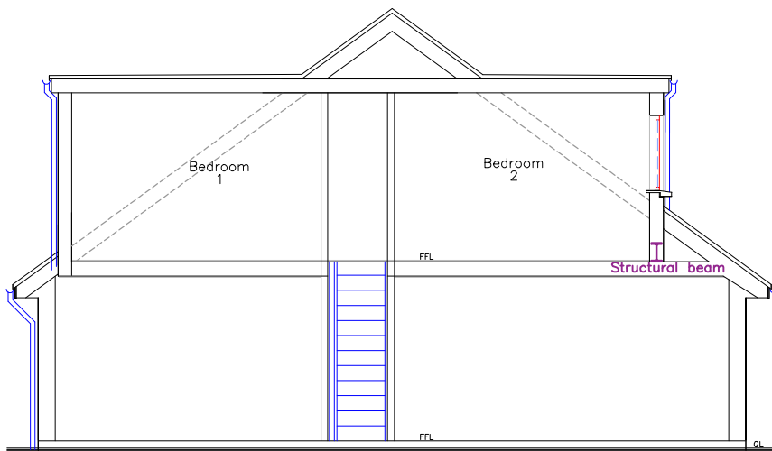
Proposed Section 1:100
