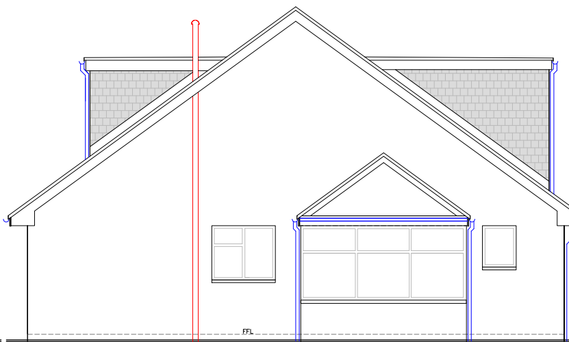
Proposed Side Elev 1:100
