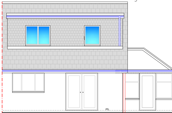
Proposed Rear Elev 1:100
