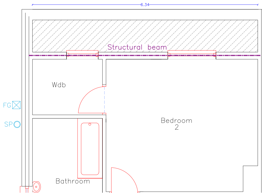
Proposed Rear Dormer Floor 1:50
