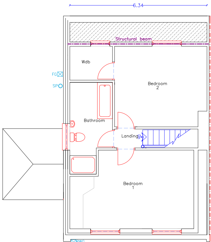
Proposed First Floor 1:100
