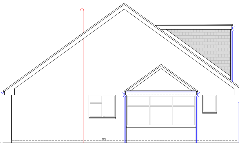
Existing Side Elev 1:100
