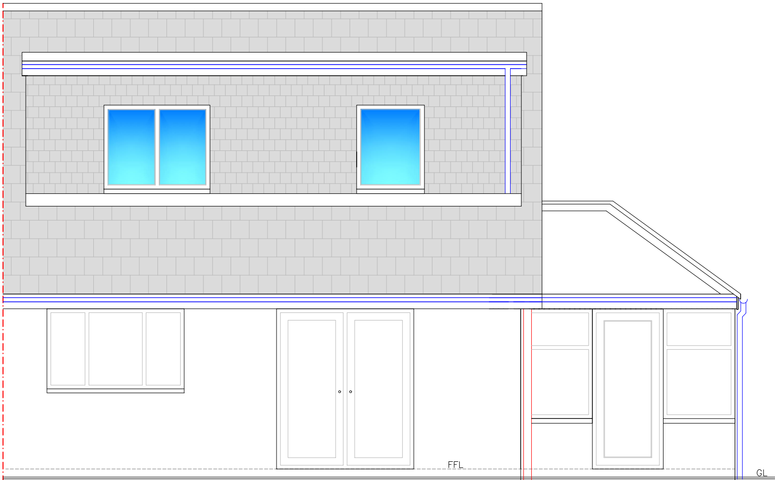
Proposed Rear Elev 1:50
