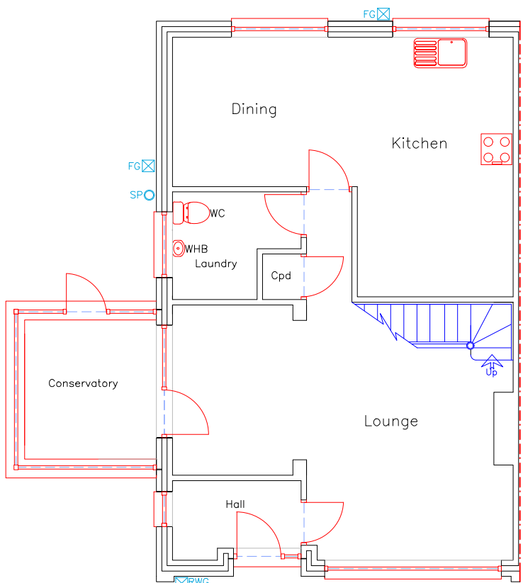
Proposed Ground Floor No change 1:100
