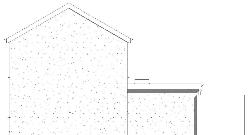
7 Existing Side 2 Elevation 1 : 100
