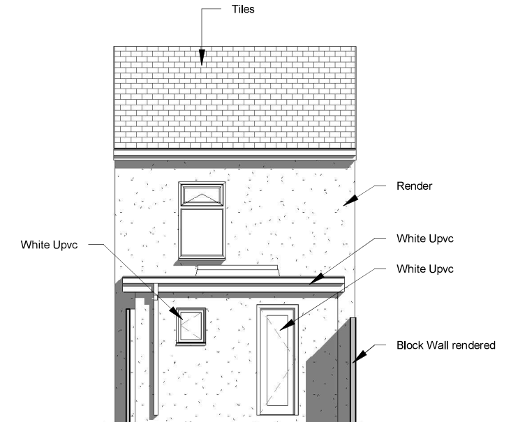
4 Existing Rear Elevation 1 : 100
