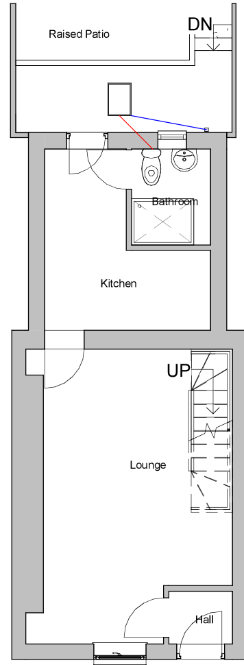
1 Existing Ground Floor 1 : 100
