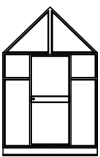
Proposed Greenhouse Side Elevation
