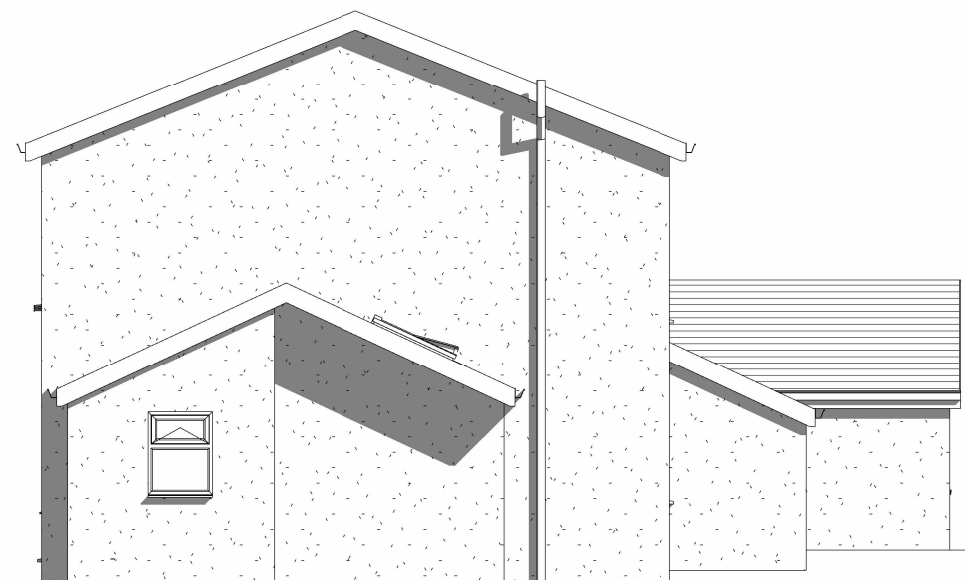
3 Existing Side 1 Elevation 1 : 100
