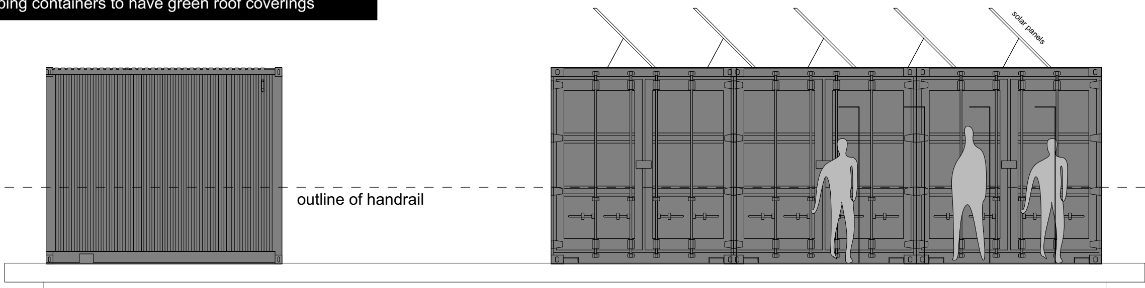
ELEVATION A WITHOUT CLADDING
