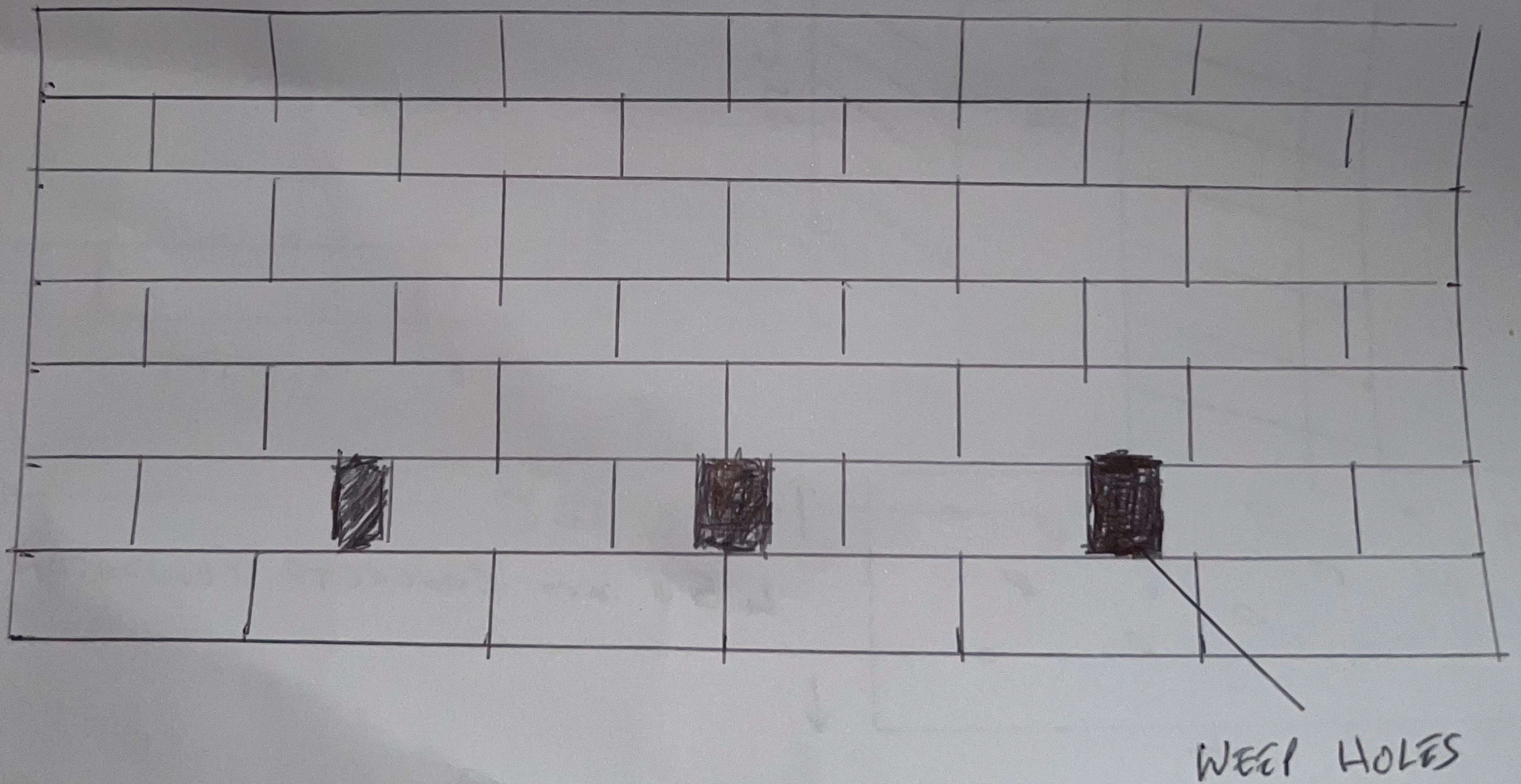
FRONT ELEVATION
