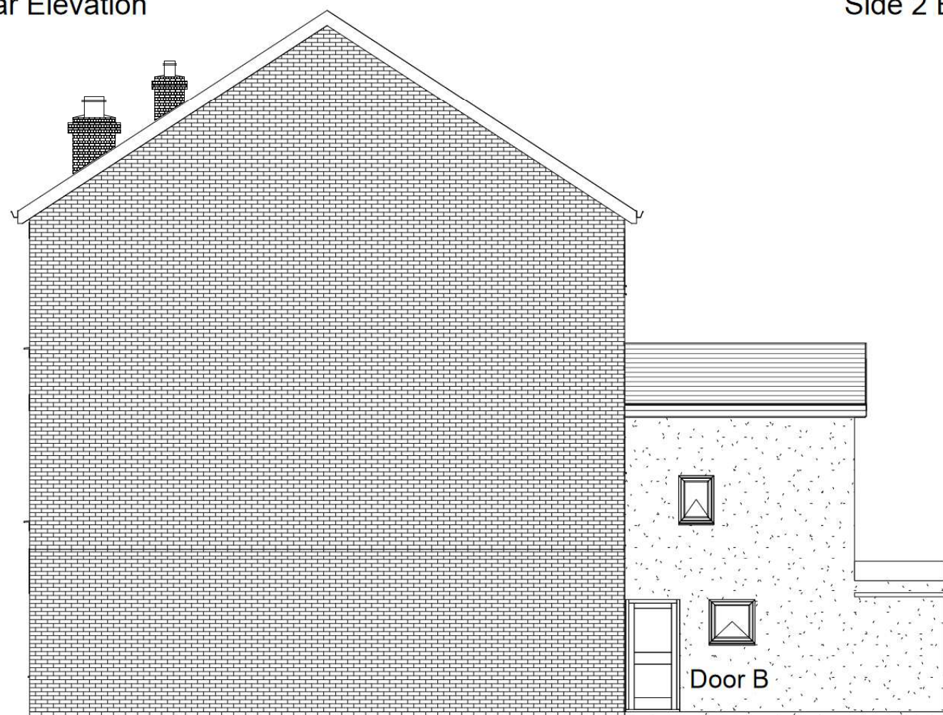
Side 1 Elevation
