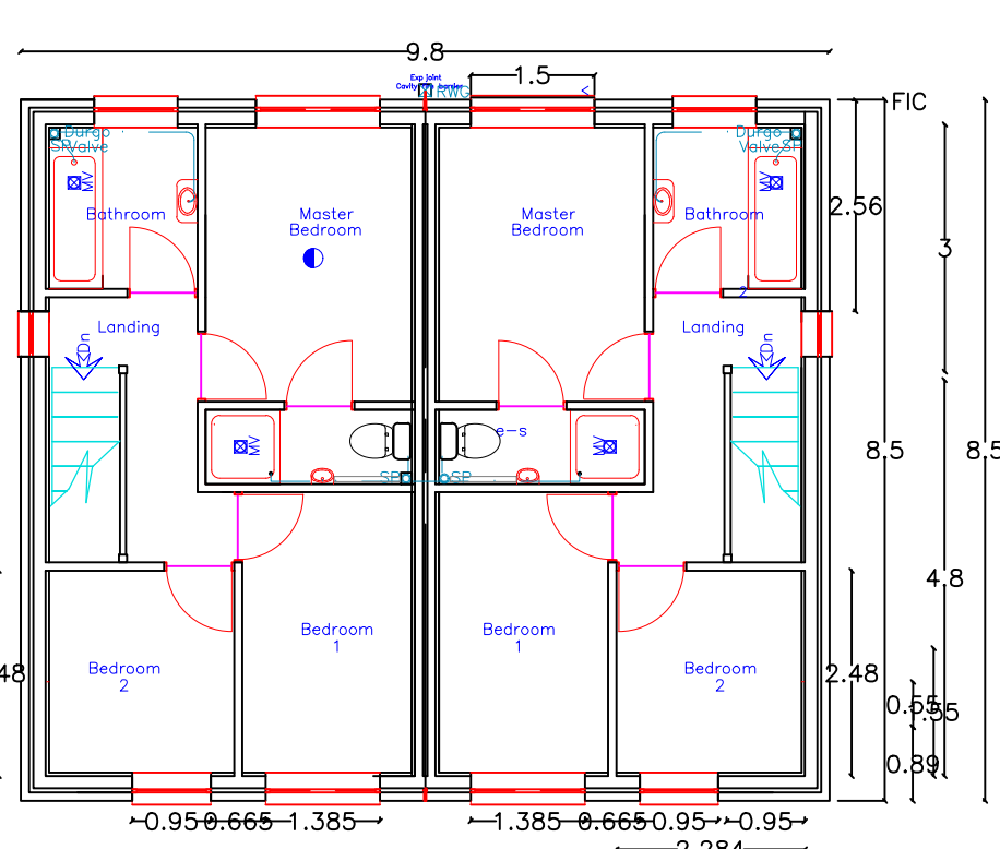
Proposed FF Plan 1:100
