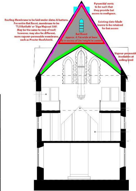
Proposed Cross Section
