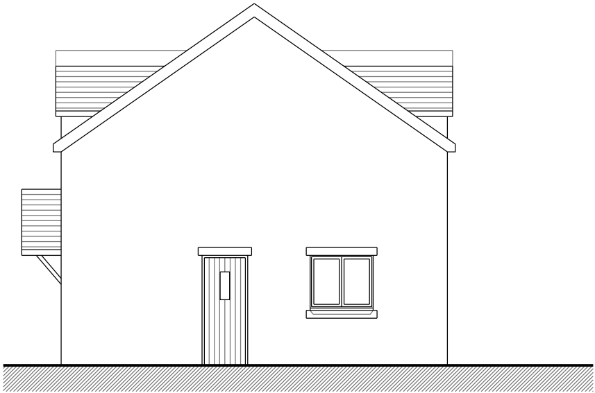
PROPOSED SIDE ELEVATION facing angus street
