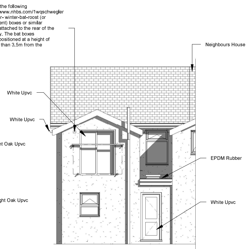
4 Proposed Rear Elevation 1 : 100
