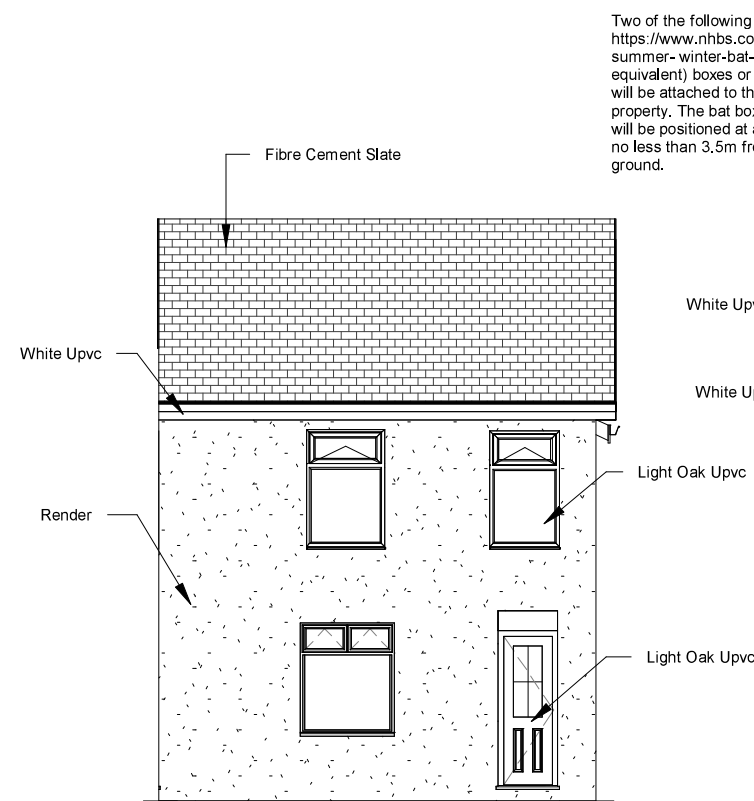
3 Proposed Front Elevation 1 : 100
