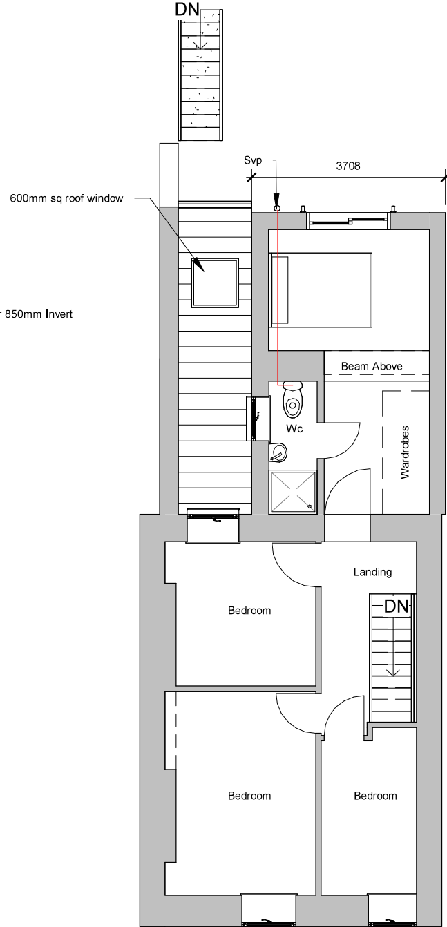
2 Proposed First Floor 1 : 100
