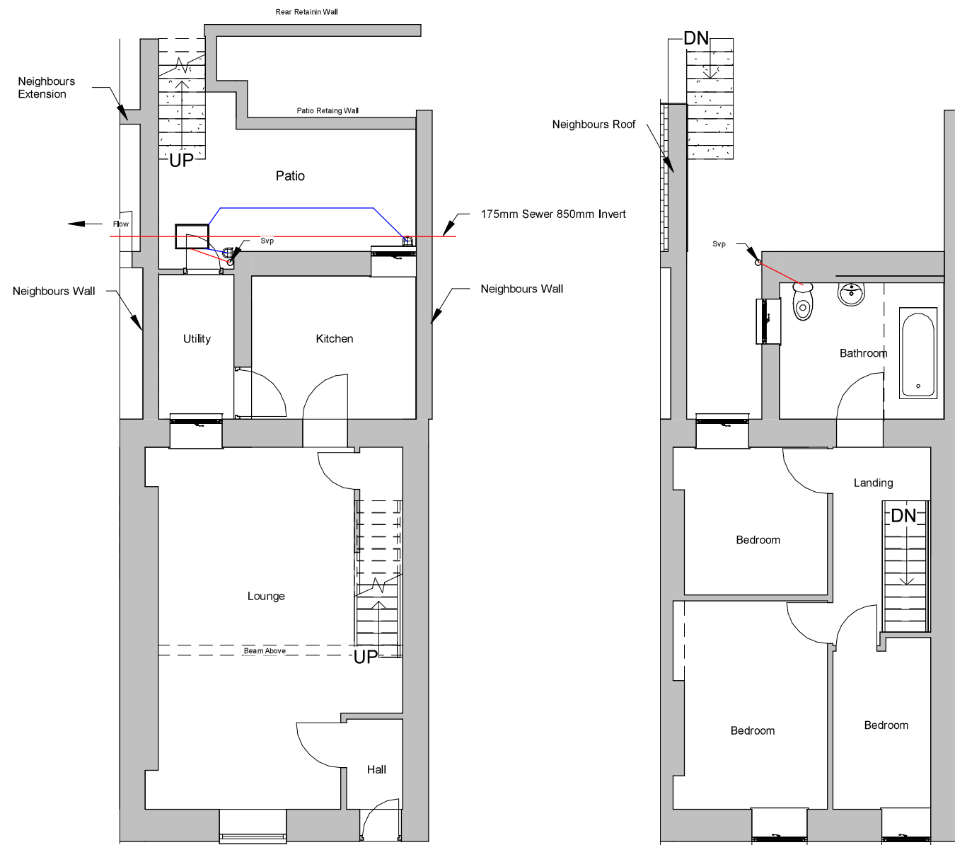
1 Existing Ground Floor 1 : 100
