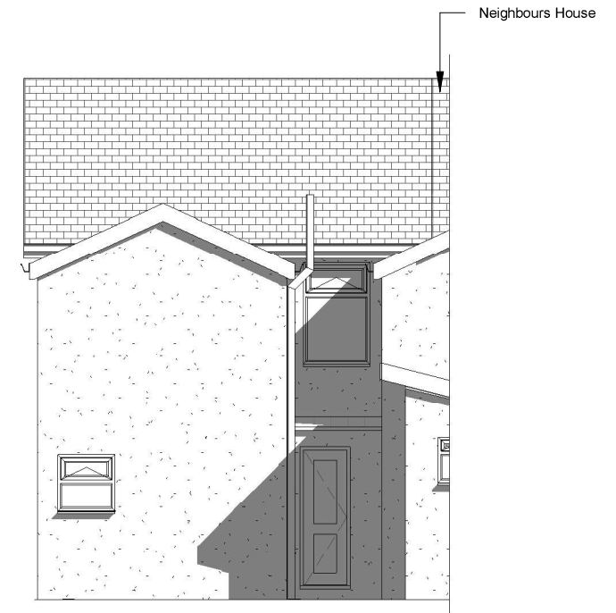
4 Existing Rear Elevation 1 : 100
