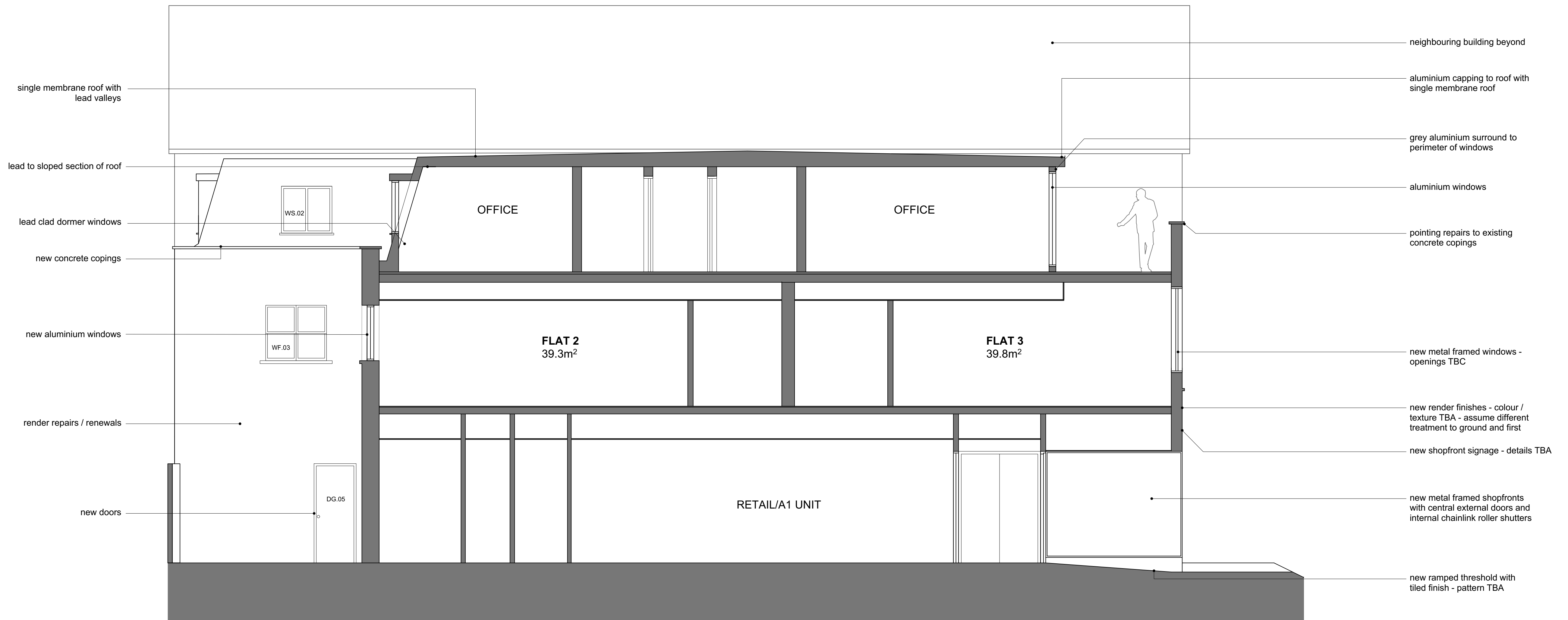
01 proposed section
