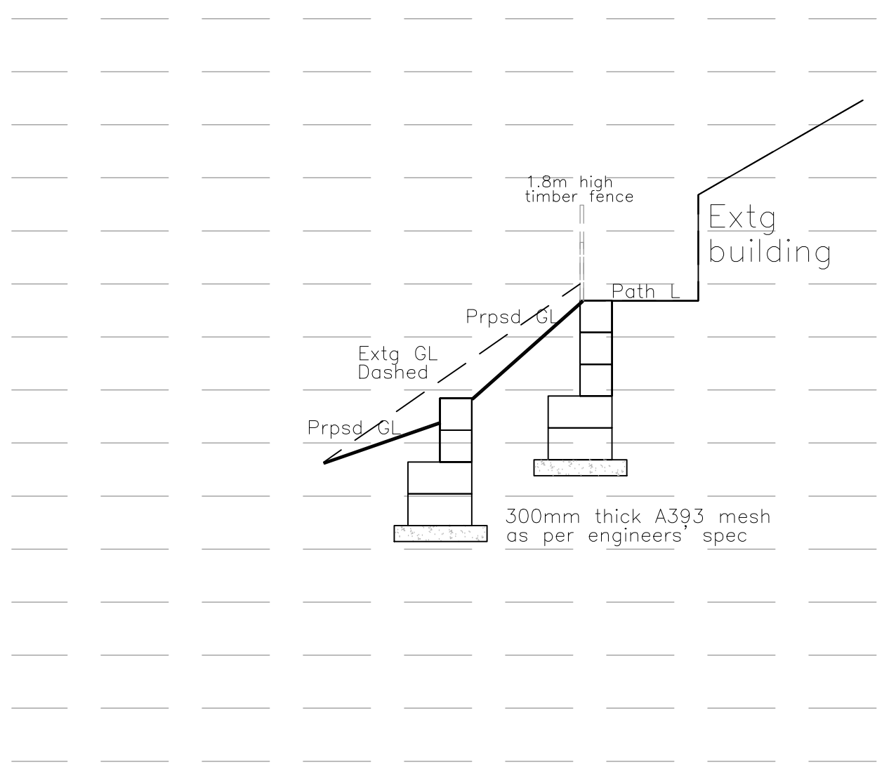
Proposed Section A-A 1:100
