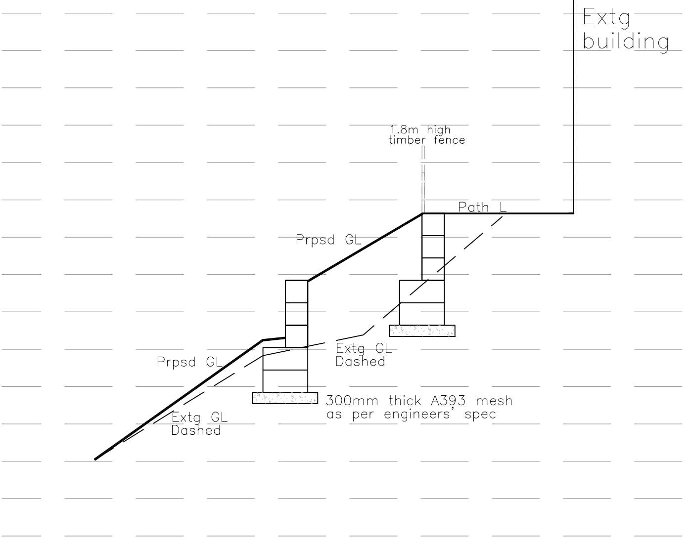
Proposed Section B-B 1:100
