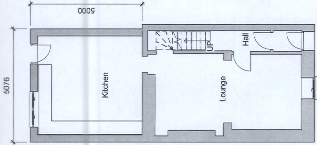
1 Proposed Ground Floor 1 : 100
