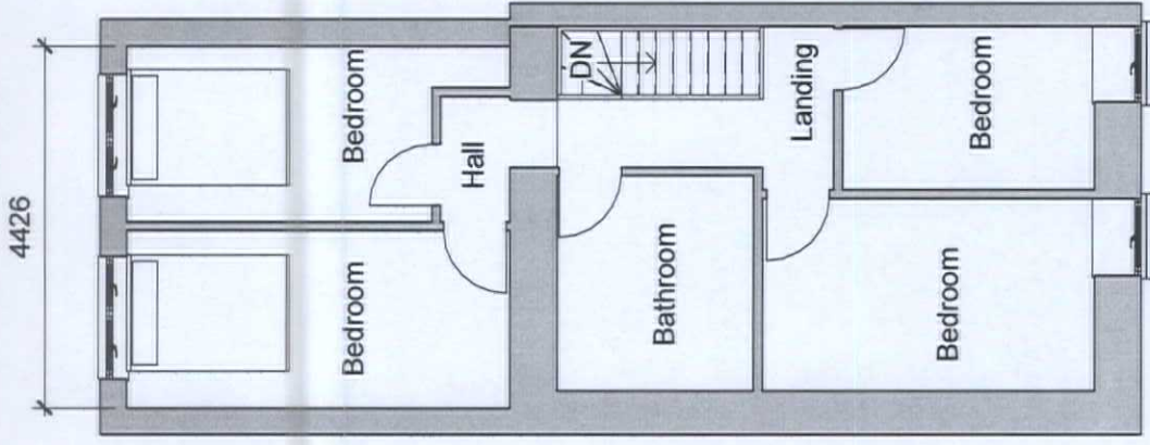
2 Proposed First Floor 1 : 100
