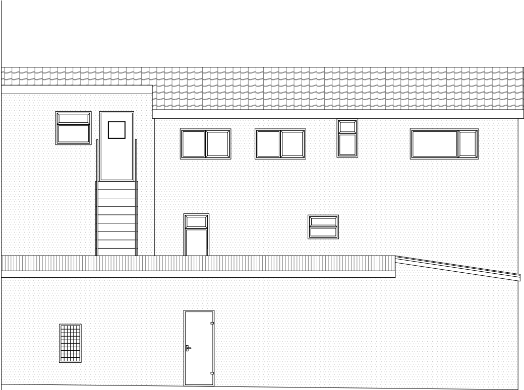
REAR ELEVATION
