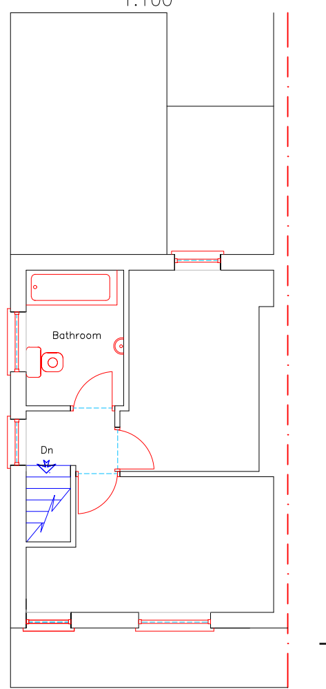
Existing First Floor Plan 1:100
