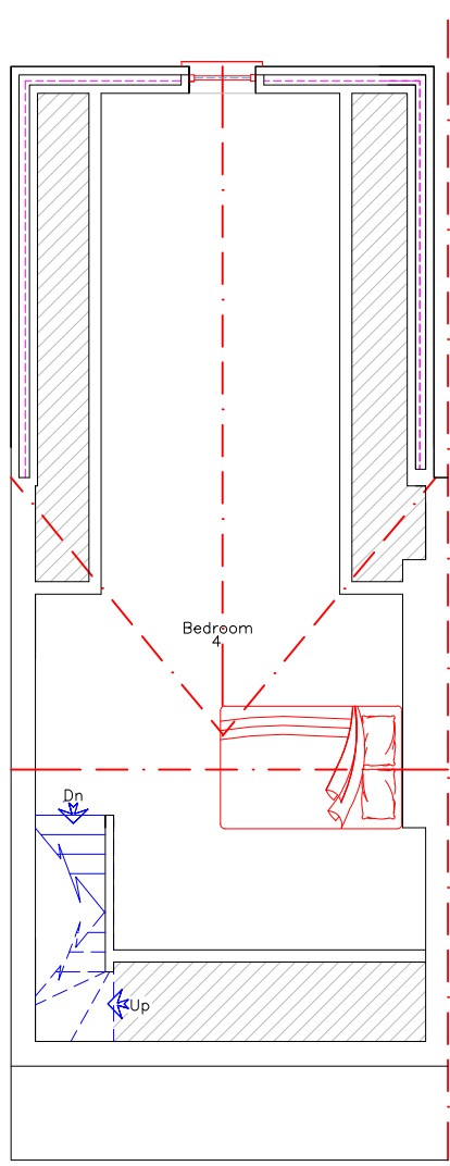
Proposed Loft Floor Plan 1:100
