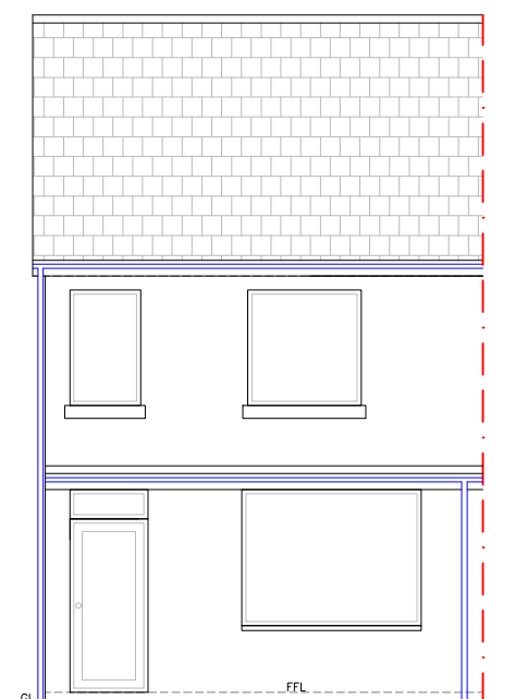
Existing Front Elev 1:100
