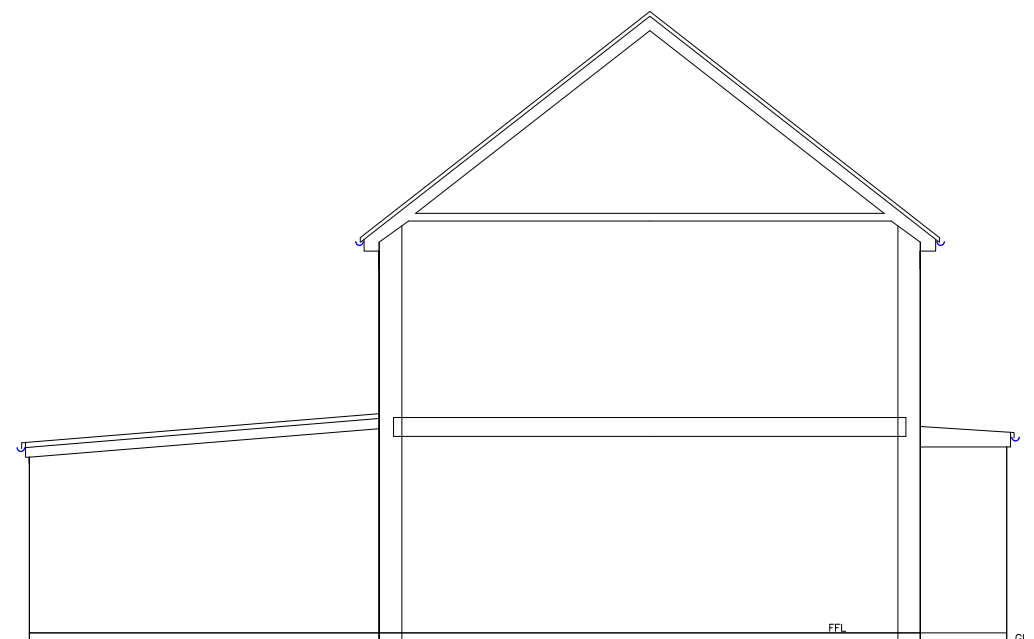
Existing Section 1:100
