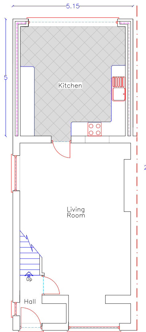
Proposed Ground Floor Plan 1:100
