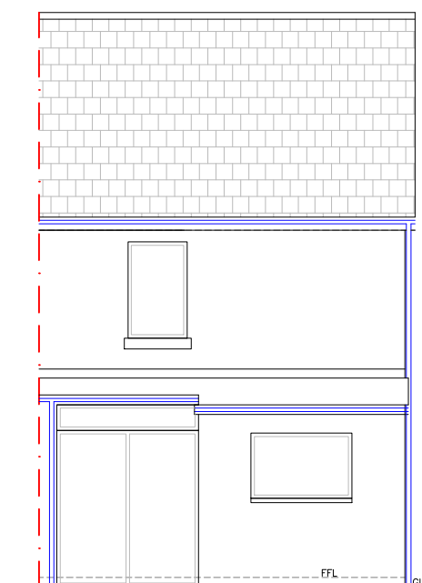
Existing Rear Elev 1:100
