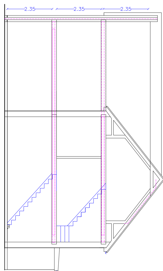
Proposed Section 1:100
