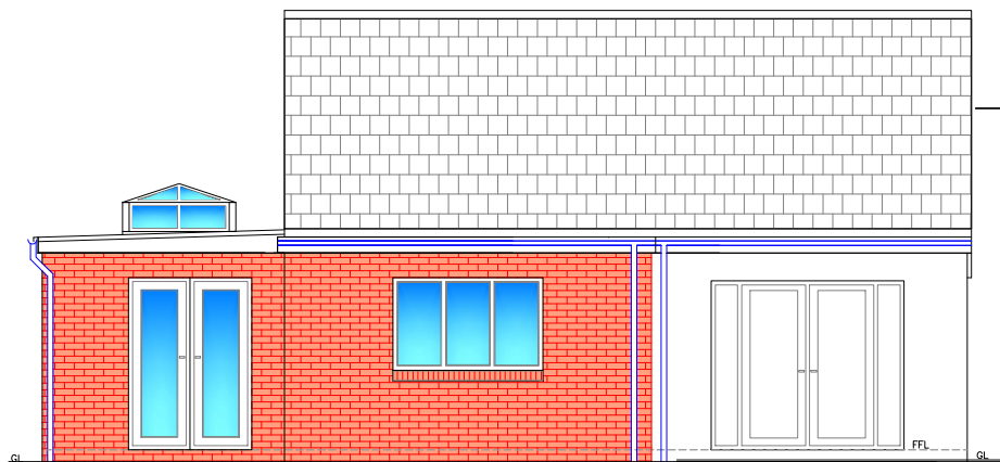
Proposed Rear Elev 1:100
