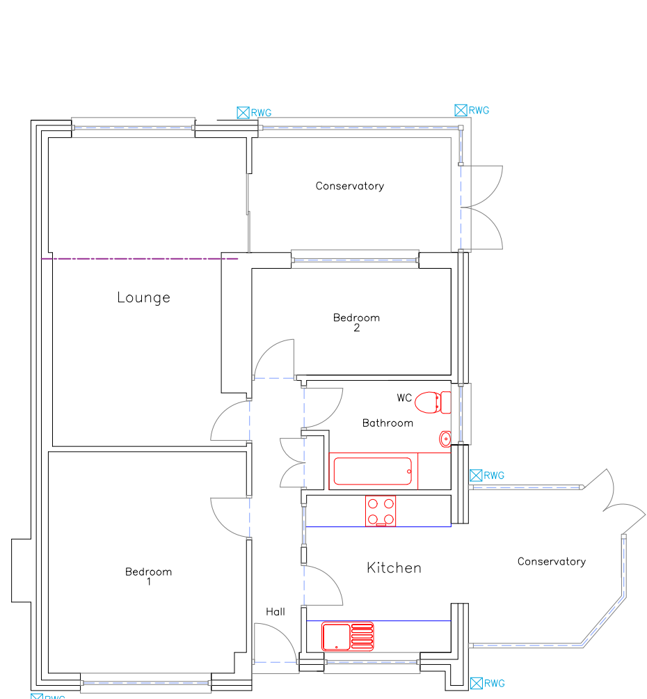
Existing Ground Floor 1:100
