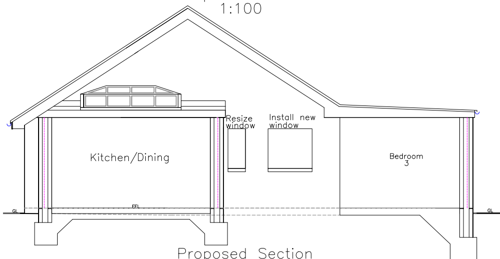
Proposed Section 1:100
