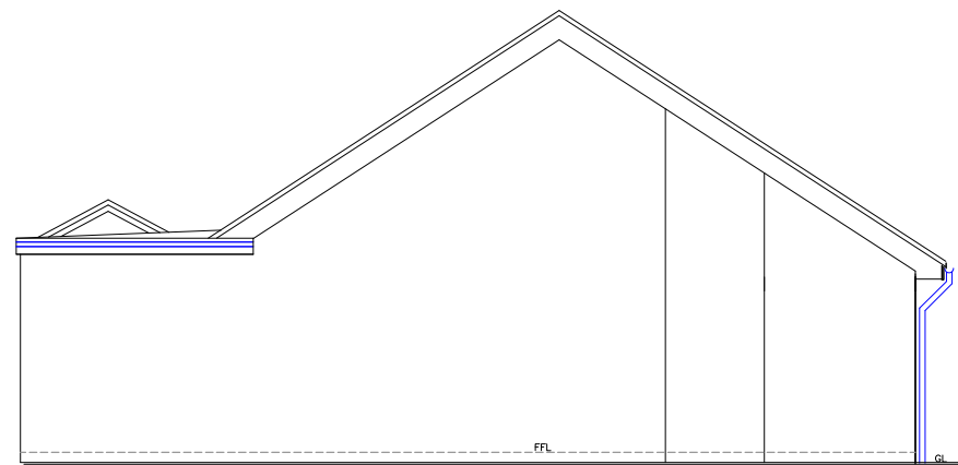
Existing Side Elev 1:100
