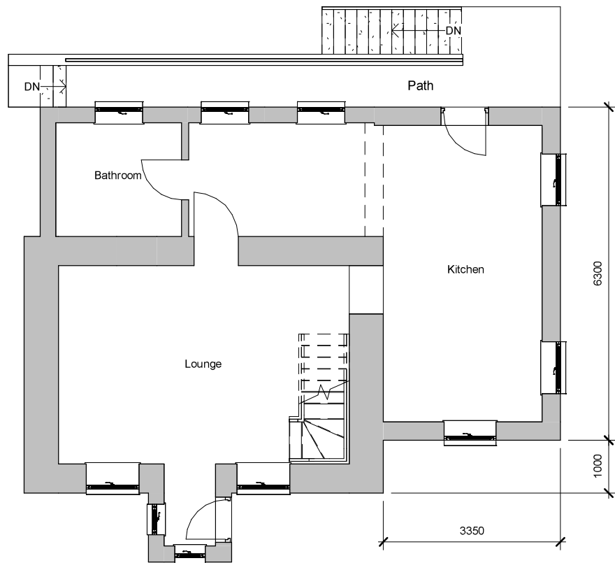
1 Proposed Ground Floor 1 : 100
